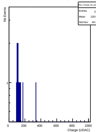
Charges in channel 94 (pong)
