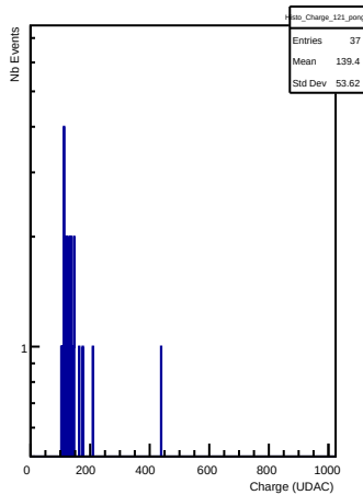
Charges in channel 121 (pong)
