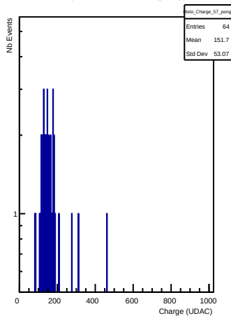
Charges in channel 57 (pong)
