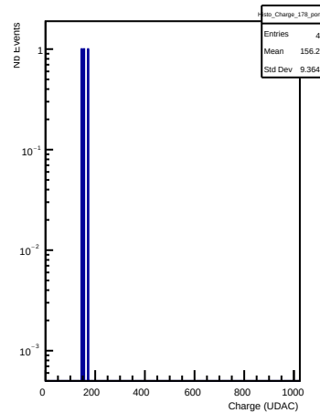
Charges in channel 178 (pong)
