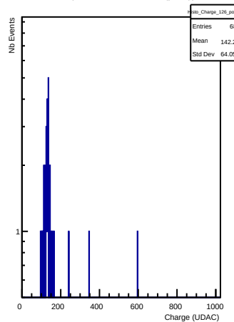
Charges in channel 126 (pong)
