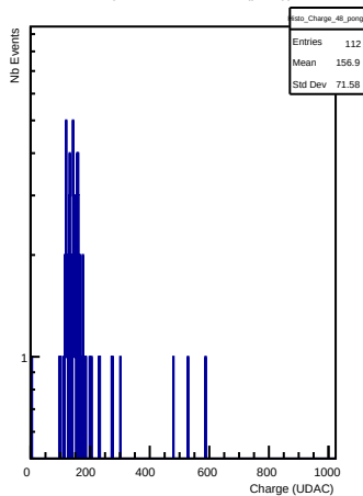
Charges in channel 48 (pong)
