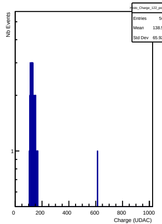
Charges in channel 122 (pong)
