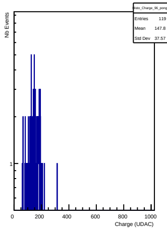
Charges in channel 96 (pong)
