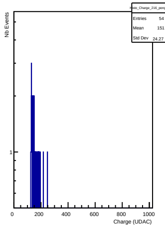
Charges in channel 216 (pong)
