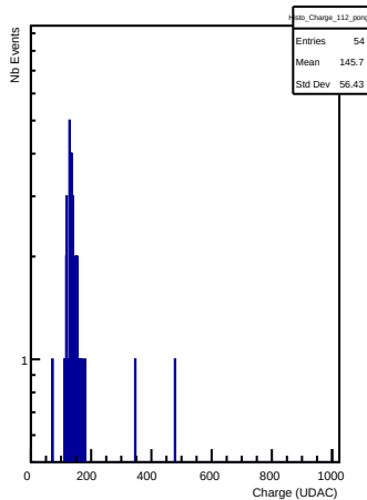
Charges in channel 112 (pong)
