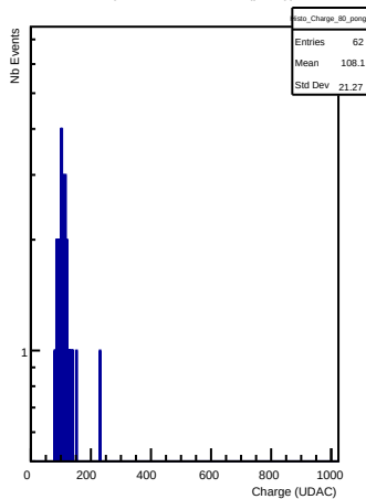
Charges in channel 80 (pong)
