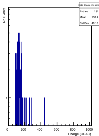
Charges in channel 25 (pong)
