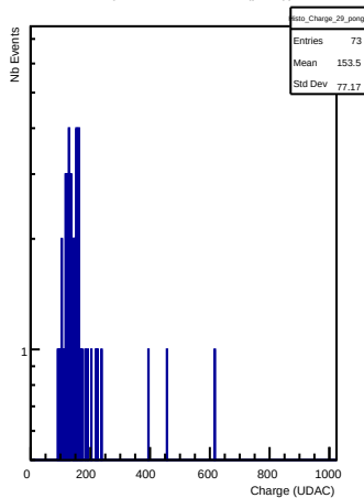
Charges in channel 29 (pong)
