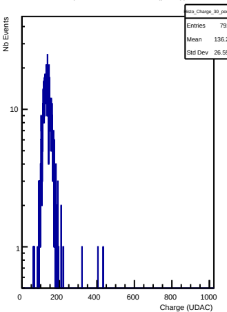
Charges in channel 30 (pong)
