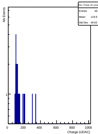
Charges in channel 84 (pong)
