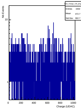
Charges in channel 128 (ping)
