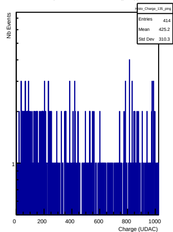
Charges in channel 135 (ping)
