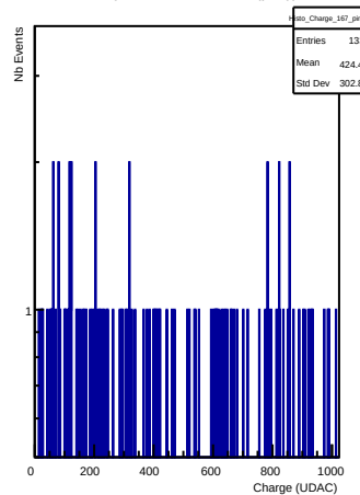
Charges in channel 167 (ping)
