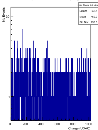
Charges in channel 148 (ping)
