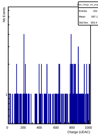
Charges in channel 161 (ping)
