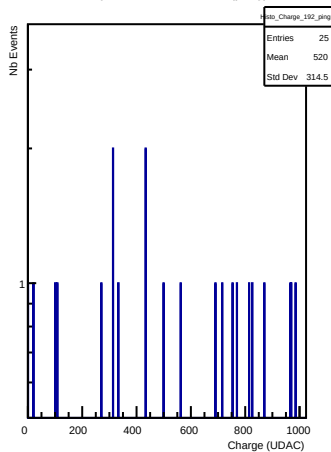
Charges in channel 192 (ping)
