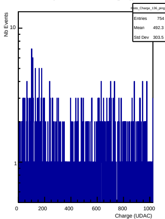
Charges in channel 136 (ping)
