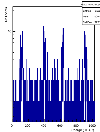
Charges in channel 155 (ping)
