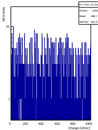
Charges in channel 152 (ping)
