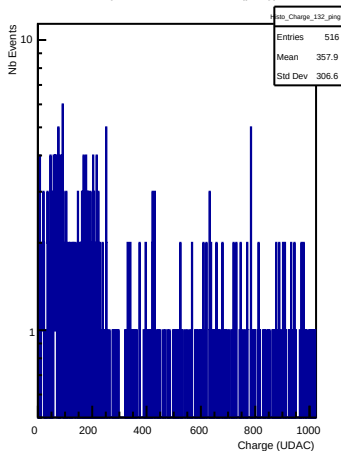
Charges in channel 132 (ping)
