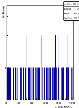
Charges in channel 174 (ping)
