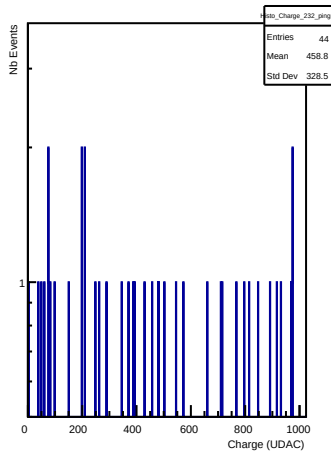
Charges in channel 232 (ping)
