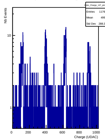
Charges in channel 147 (ping)
