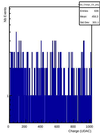
Charges in channel 131 (ping)
