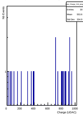
Charges in channel 216 (ping)
