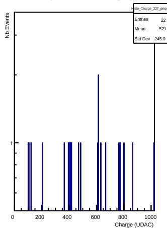
Charges in channel 227 (ping)
