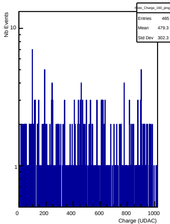
Charges in channel 160 (ping)
