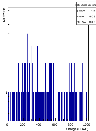
Charges in channel 208 (ping)
