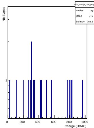
Charges in channel 200 (ping)
