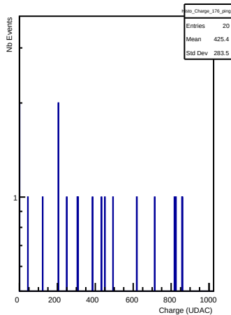
Charges in channel 176 (ping)
