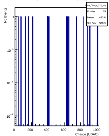
Charges in channel 223 (ping)
