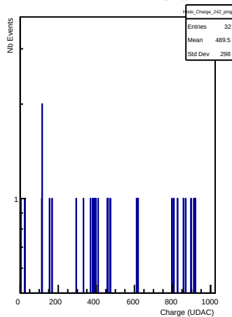
Charges in channel 242 (ping)
