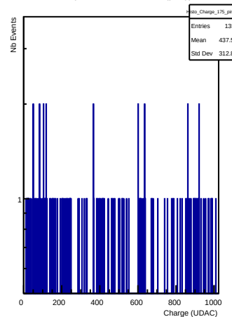
Charges in channel 175 (ping)
