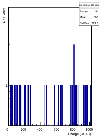
Charges in channel 225 (ping)
