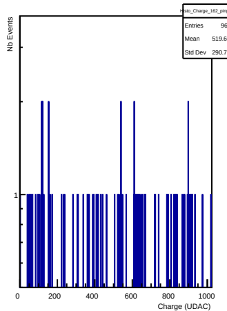
Charges in channel 162 (ping)
