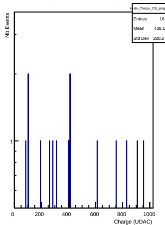
Charges in channel 226 (ping)
