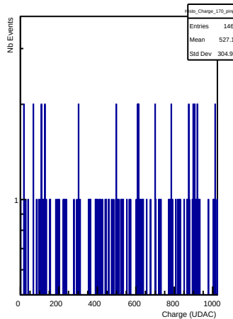
Charges in channel 170 (ping)
