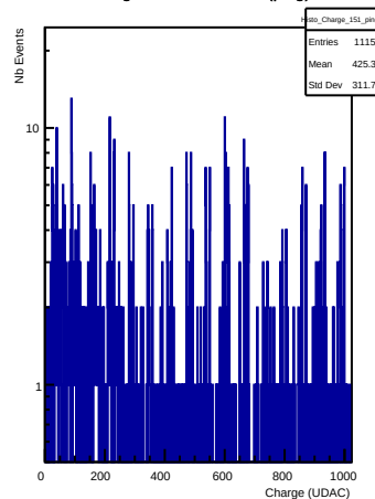
Charges in channel 151 (ping)
