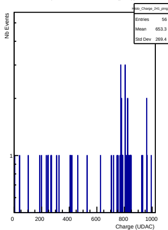
Charges in channel 241 (ping)
