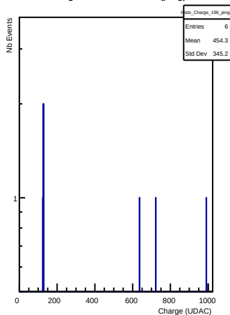
Charges in channel 196 (ping)
