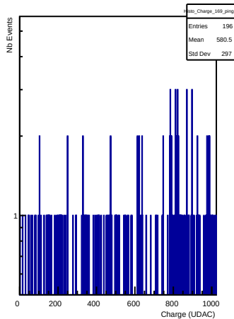
Charges in channel 169 (ping)
