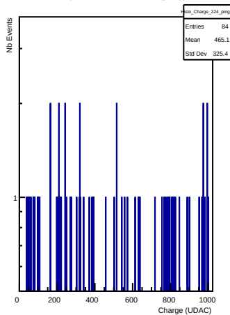
Charges in channel 224 (ping)
