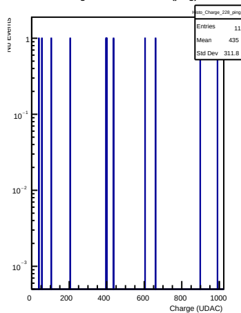
Charges in channel 228 (ping)
