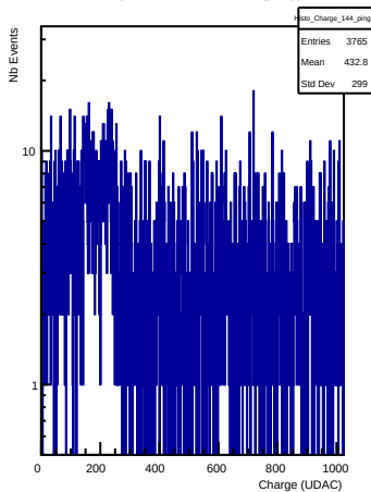
Charges in channel 144 (ping)
