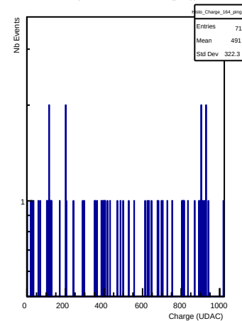
Charges in channel 164 (ping)
