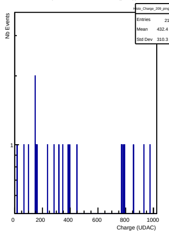
Charges in channel 209 (ping)
