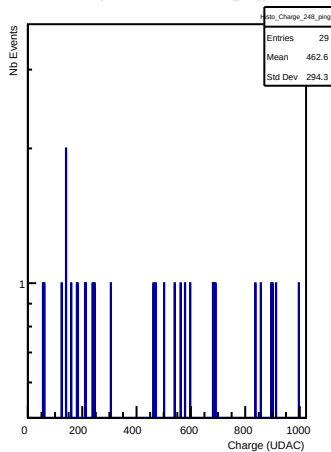
Charges in channel 248 (ping)
