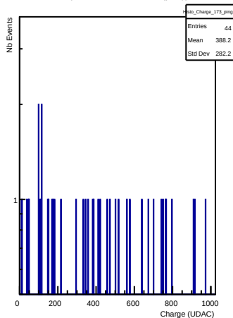
Charges in channel 173 (ping)
