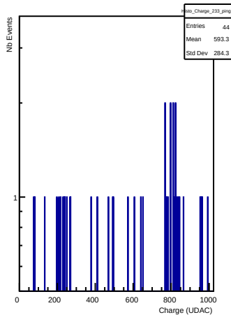
Charges in channel 233 (ping)
