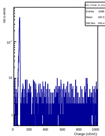
Charges in channel 24 (ping)
