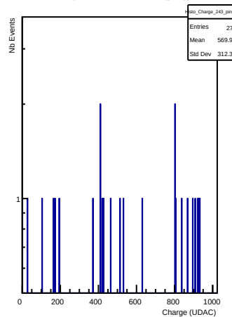
Charges in channel 243 (ping)
