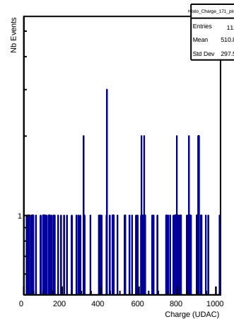
Charges in channel 171 (ping)
