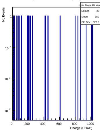
Charges in channel 231 (ping)
