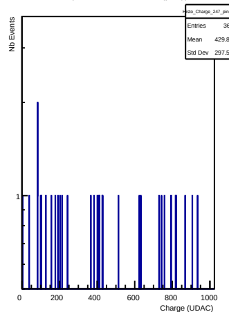
Charges in channel 247 (ping)
