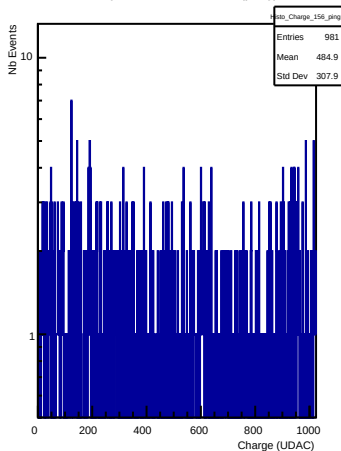
Charges in channel 156 (ping)
