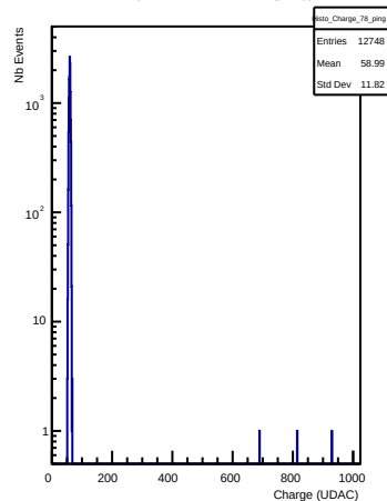
Charges in channel 78 (ping)
