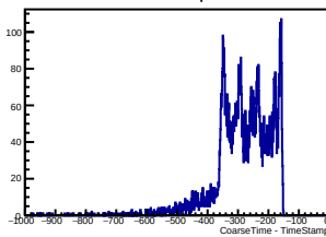
CT - Time stamp Chn101
