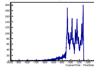
CT - Time stamp Chn47
