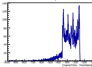
CT - Time stamp Chn106
