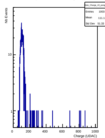
Charges in channel 43 (pong)
