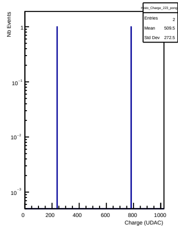
Charges in channel 223 (pong)
