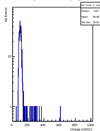
Charges in channel 47 (pong)
