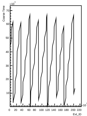
Coarse_times wrt Evt_ID for channel 126 (pong)
