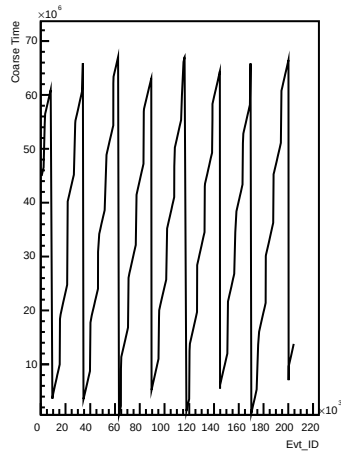
Coarse_times wrt Evt_ID for channel 67 (pong)
