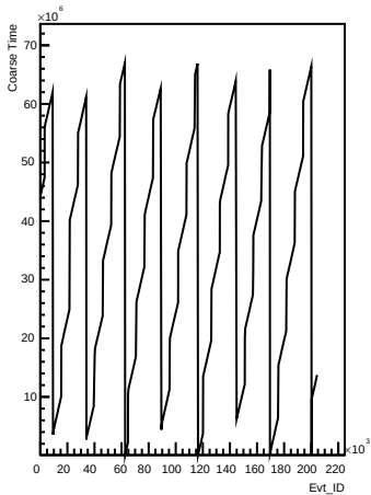
Coarse_times wrt Evt_ID for channel 93 (pong)
