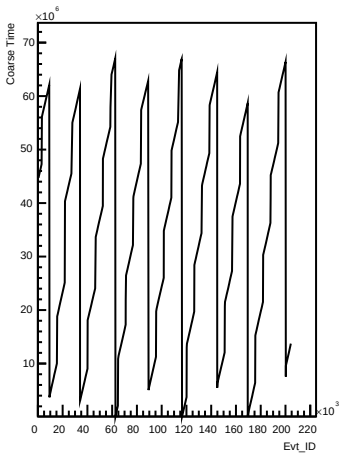
Coarse_times wrt Evt_ID for channel 36 (pong)
