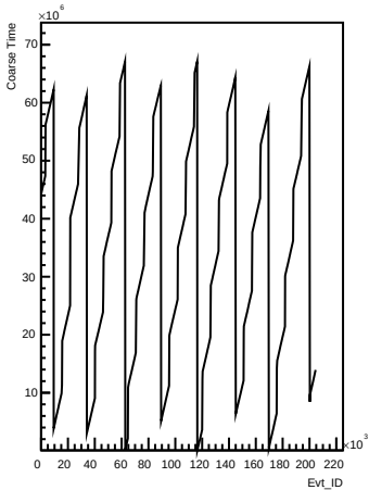
Coarse_times wrt Evt_ID for channel 84 (pong)
