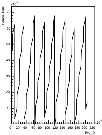
Coarse_times wrt Evt_ID for channel 120 (pong)
