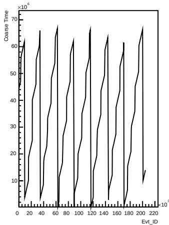
Coarse_times wrt Evt_ID for channel 113 (pong)
