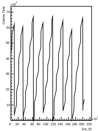
Coarse_times wrt Evt_ID for channel 78 (pong)
