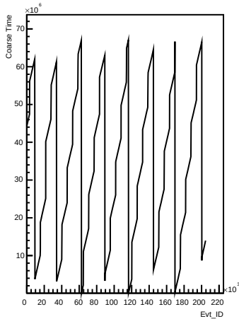
Coarse_times wrt Evt_ID for channel 85 (pong)
