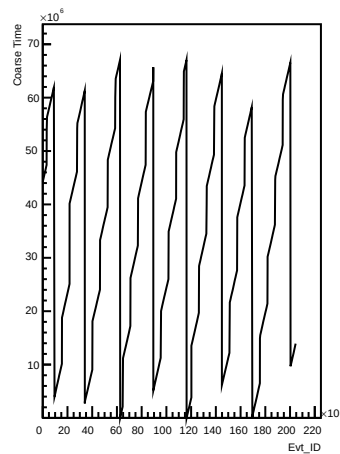
Coarse_times wrt Evt_ID for channel 59 (pong)
