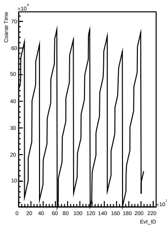
Coarse_times wrt Evt_ID for channel 109 (pong)
