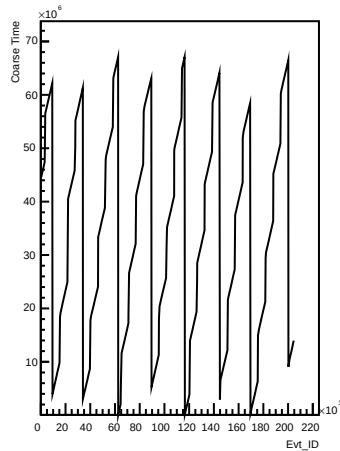
Coarse_times wrt Evt_ID for channel 114 (pong)
