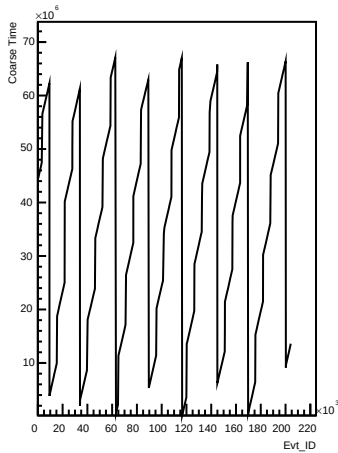
Coarse_times wrt Evt_ID for channel 5 (pong)
