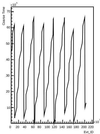
Coarse_times wrt Evt_ID for channel 17 (pong)
