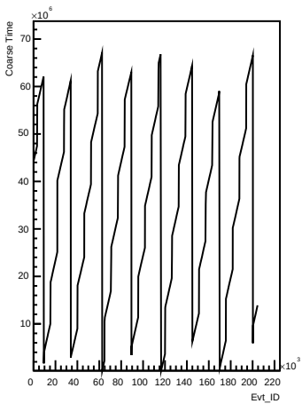
Coarse_times wrt Evt_ID for channel 12 (pong)
