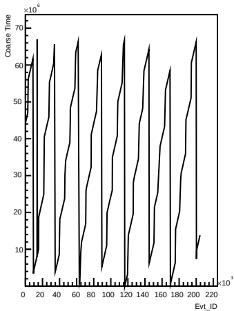
Coarse_times wrt Evt_ID for channel 65 (pong)
