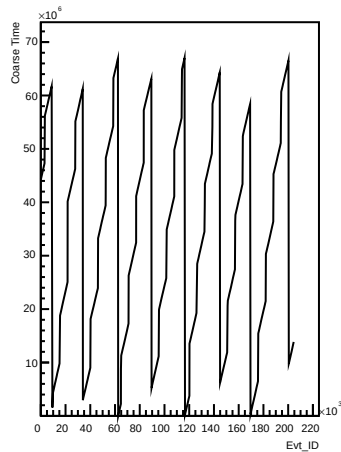
Coarse_times wrt Evt_ID for channel 50 (pong)
