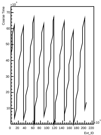
Coarse_times wrt Evt_ID for channel 53 (pong)
