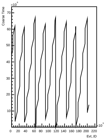
Coarse_times wrt Evt_ID for channel 116 (pong)
