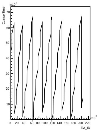
Coarse_times wrt Evt_ID for channel 35 (pong)
