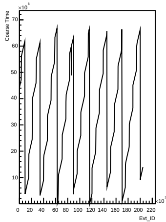
Coarse_times wrt Evt_ID for channel 6 (pong)
