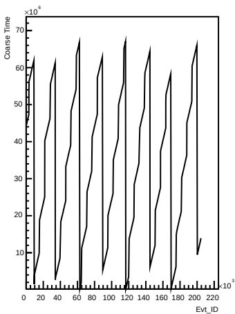
Coarse_times wrt Evt_ID for channel 56 (pong)
