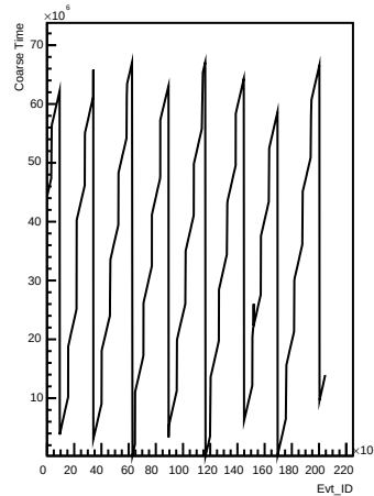
Coarse_times wrt Evt_ID for channel 87 (pong)
