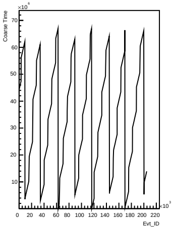
Coarse_times wrt Evt_ID for channel 44 (pong)
