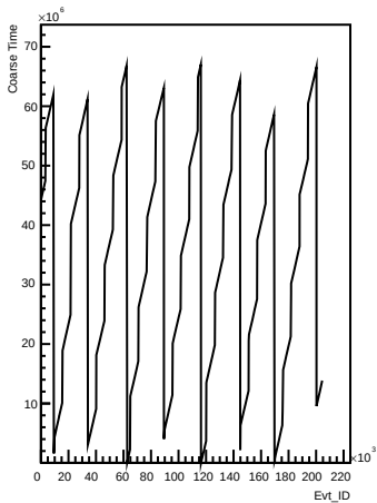
Coarse_times wrt Evt_ID for channel 49 (pong)
