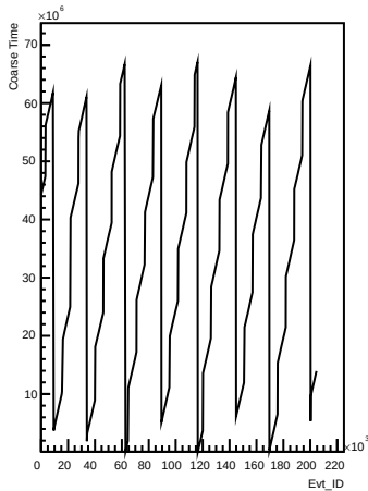
Coarse_times wrt Evt_ID for channel 43 (pong)
