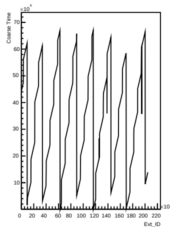
Coarse_times wrt Evt_ID for channel 63 (pong)
