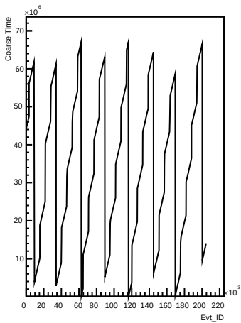
Coarse_times wrt Evt_ID for channel 13 (pong)
