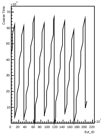
Coarse_times wrt Evt_ID for channel 47 (pong)
