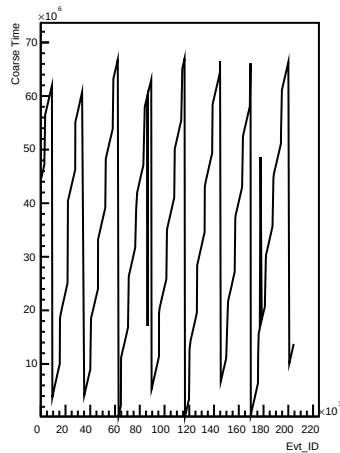
Coarse_times wrt Evt_ID for channel 23 (pong)
