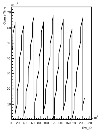
Coarse_times wrt Evt_ID for channel 10 (pong)
