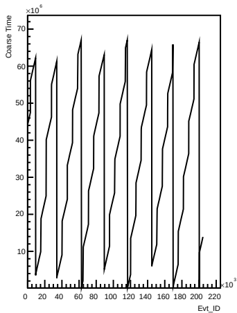
Coarse_times wrt Evt_ID for channel 88 (pong)
