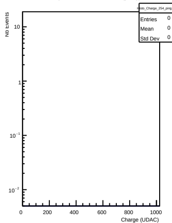
Charges in channel 254 (ping)
