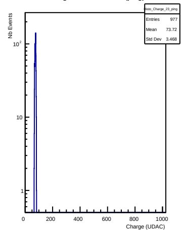
Charges in channel 23 (ping)
