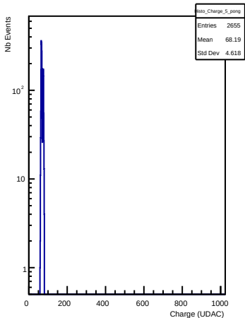
Charges in channel 5 (pong)
