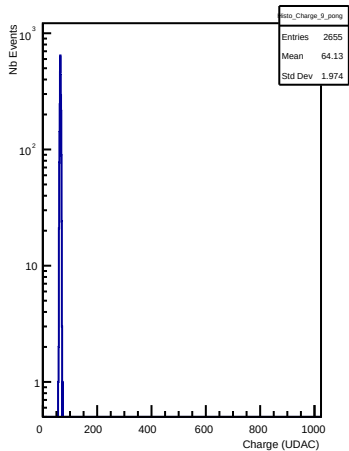
Charges in channel 9 (pong)
