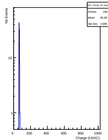
Charges in channel 99 (pong)
