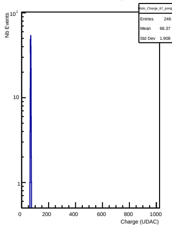
Charges in channel 67 (pong)
