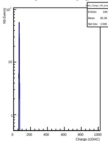
Charges in channel 103 (pong)
