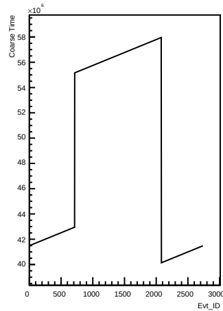
Coarse_times wrt Evt_ID for channel 14 (pong)
