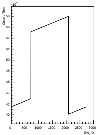
Coarse_times wrt Evt_ID for channel 9 (pong)
