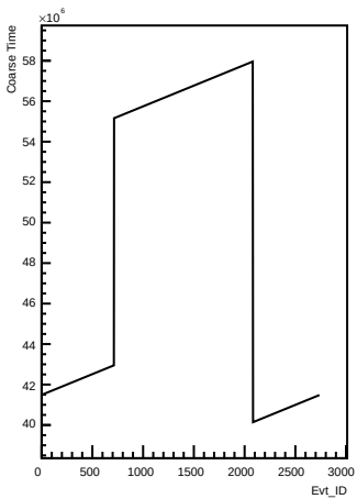
Coarse_times wrt Evt_ID for channel 0 (pong)
