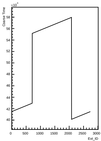
Coarse_times wrt Evt_ID for channel 2 (pong)
