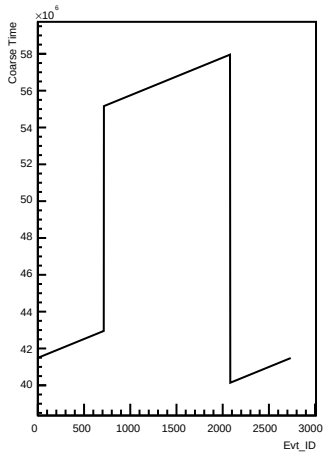
Coarse_times wrt Evt_ID for channel 13 (pong)
