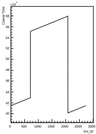
Coarse_times wrt Evt_ID for channel 5 (pong)
