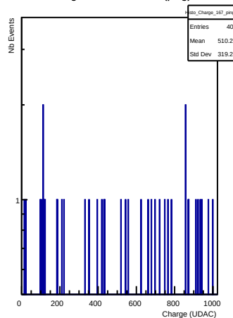
Charges in channel 167 (ping)
