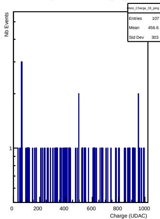
Charges in channel 33 (ping)
