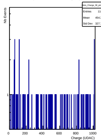
Charges in channel 38 (ping)
