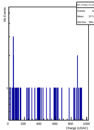
Charges in channel 34 (ping)
