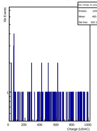
Charges in channel 43 (ping)
