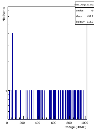
Charges in channel 36 (ping)
