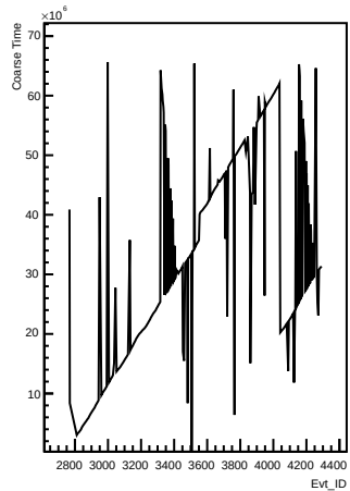
Coarse_times wrt Evt_ID for channel 51 (pong)
