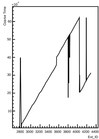
Coarse_times wrt Evt_ID for channel 75 (pong)
