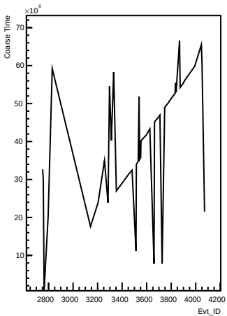
Coarse_times wrt Evt_ID for channel 88 (pong)
