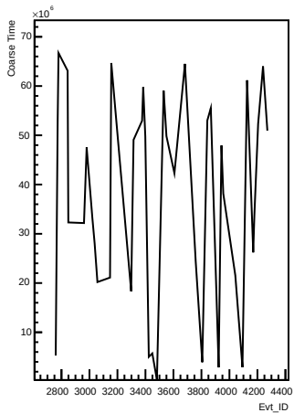
Coarse_times wrt Evt_ID for channel 113 (pong)
