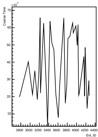
Coarse_times wrt Evt_ID for channel 119 (pong)
