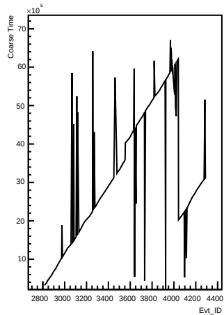
Coarse_times wrt Evt_ID for channel 55 (pong)
