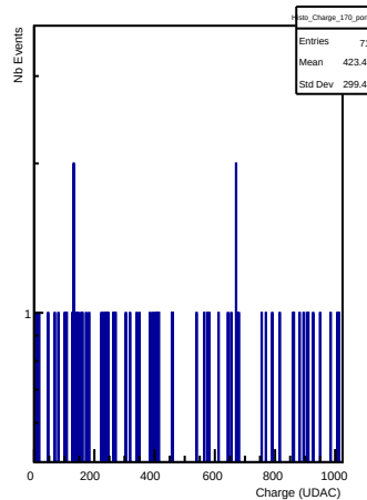
Charges in channel 170 (pong)
