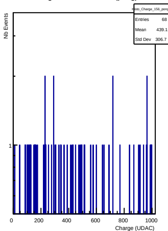
Charges in channel 156 (pong)
