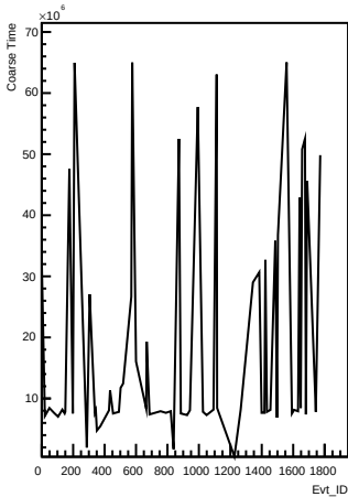
Coarse_times wrt Evt_ID for channel 172 (pong)
