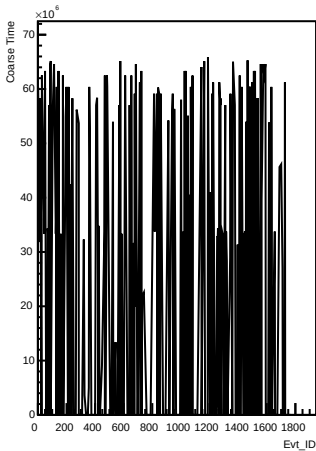
Coarse_times wrt Evt_ID for channel 160 (pong)
