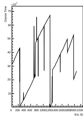
Coarse_times wrt Evt_ID for channel 99 (pong)
