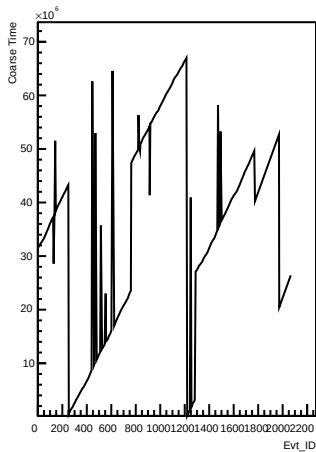
Coarse_times wrt Evt_ID for channel 49 (pong)
