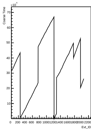
Coarse_times wrt Evt_ID for channel 78 (pong)
