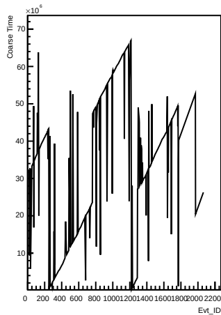
Coarse_times wrt Evt_ID for channel 59 (pong)
