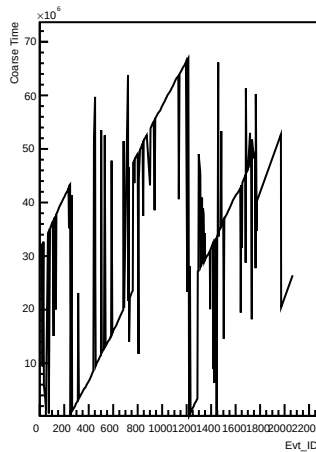
Coarse_times wrt Evt_ID for channel 51 (pong)
