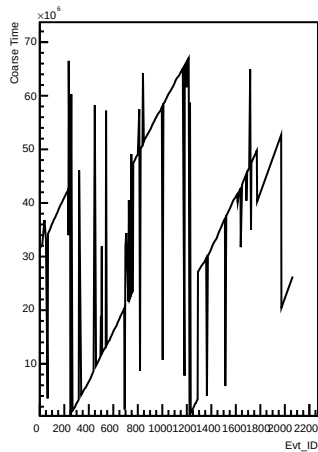
Coarse_times wrt Evt_ID for channel 58 (pong)
