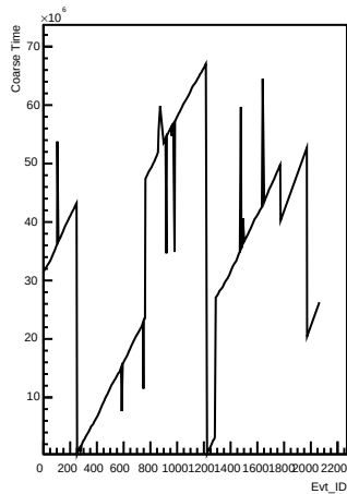
Coarse_times wrt Evt_ID for channel 62 (pong)
