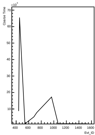
Coarse_times wrt Evt_ID for channel 217 (pong)
