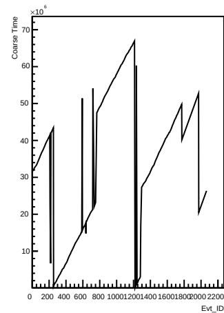
Coarse_times wrt Evt_ID for channel 103 (pong)
