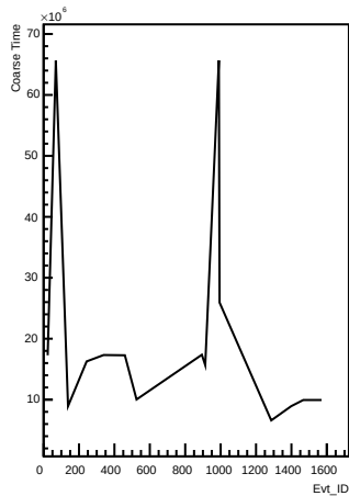
Coarse_times wrt Evt_ID for channel 251 (pong)
