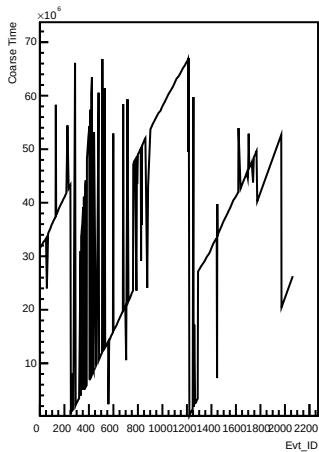
Coarse_times wrt Evt_ID for channel 56 (pong)
