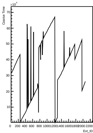
Coarse_times wrt Evt_ID for channel 57 (pong)
