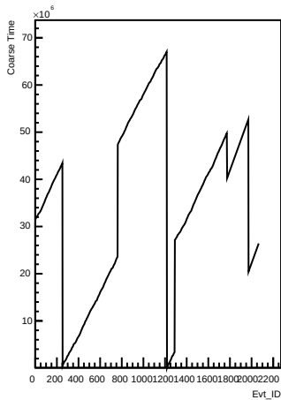
Coarse_times wrt Evt_ID for channel 12 (pong)
