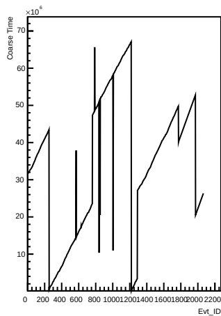
Coarse_times wrt Evt_ID for channel 75 (pong)
