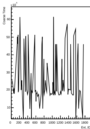
Coarse_times wrt Evt_ID for channel 151 (pong)
