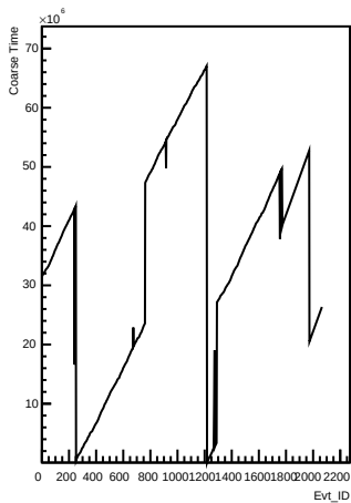
Coarse_times wrt Evt_ID for channel 77 (pong)
