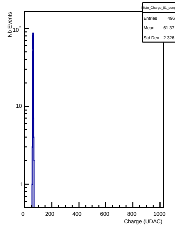
Charges in channel 81 (pong)
