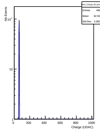
Charges in channel 86 (pong)
