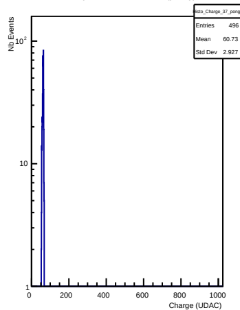
Charges in channel 37 (pong)
