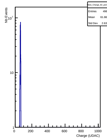
Charges in channel 82 (pong)
