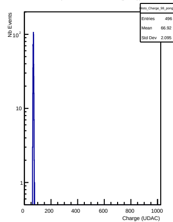
Charges in channel 98 (pong)
