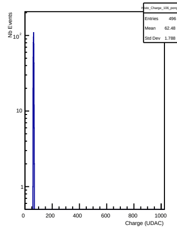
Charges in channel 106 (pong)
