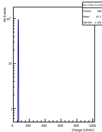
Charges in channel 33 (pong)
