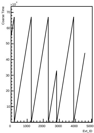
Coarse_times wrt Evt_ID for channel 4 (ping)
