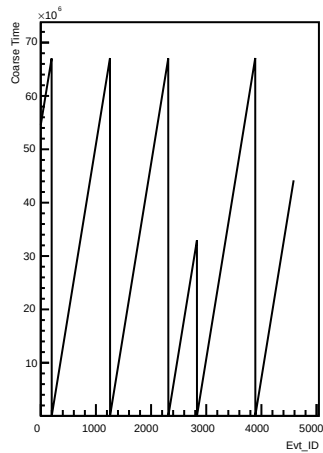
Coarse_times wrt Evt_ID for channel 11 (ping)
