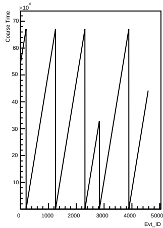
Coarse_times wrt Evt_ID for channel 15 (ping)
