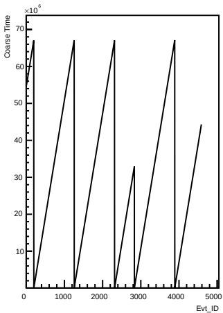
Coarse_times wrt Evt_ID for channel 0 (ping)
