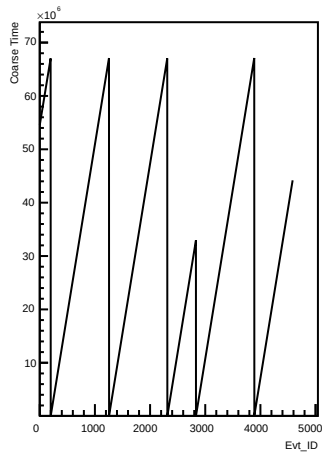
Coarse_times wrt Evt_ID for channel 3 (ping)
