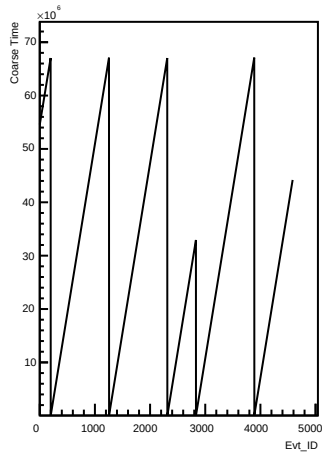
Coarse_times wrt Evt_ID for channel 7 (ping)
