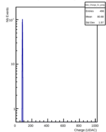
Charges in channel 51 (pong)
