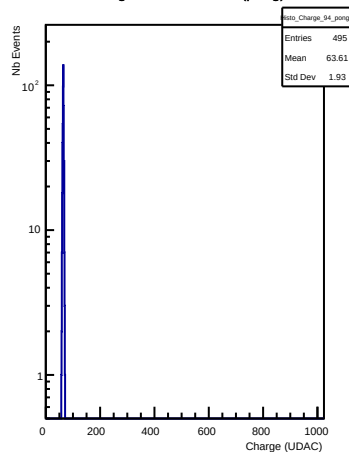
Charges in channel 94 (pong)
