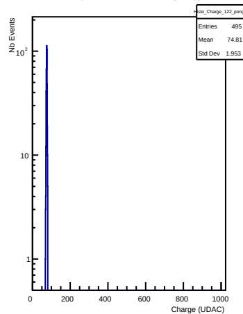
Charges in channel 122 (pong)
