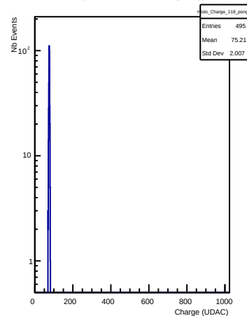
Charges in channel 118 (pong)
