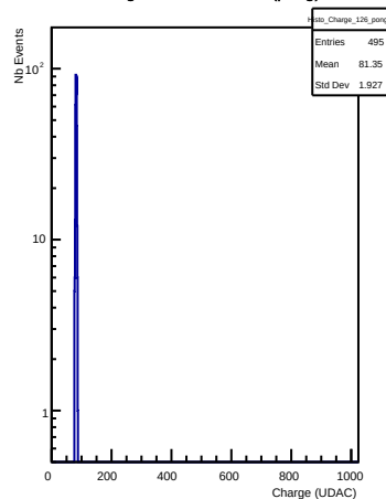
Charges in channel 126 (pong)
