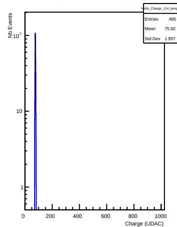
Charges in channel 114 (pong)
