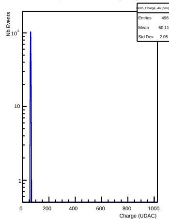
Charges in channel 46 (pong)
