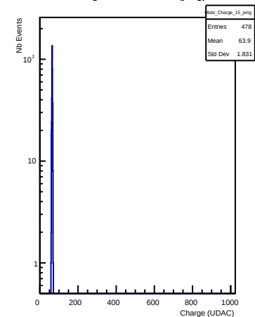
Charges in channel 15 (ping)
