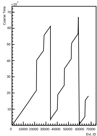
Coarse_times wrt Evt_ID for channel 71 (pong)
