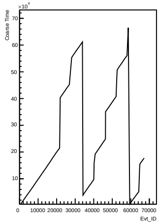
Coarse_times wrt Evt_ID for channel 67 (pong)
