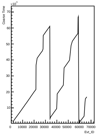
Coarse_times wrt Evt_ID for channel 65 (pong)
