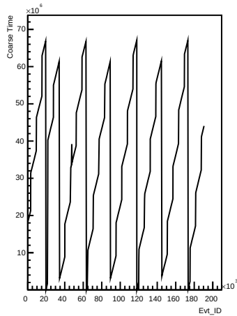
Coarse_times wrt Evt_ID for channel 94 (ping)
