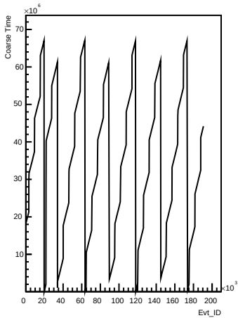
Coarse_times wrt Evt_ID for channel 93 (ping)
