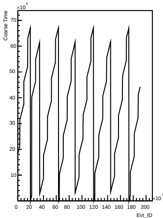
Coarse_times wrt Evt_ID for channel 61 (ping)
