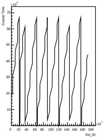
Coarse_times wrt Evt_ID for channel 92 (ping)
