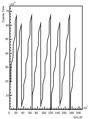
Coarse_times wrt Evt_ID for channel 78 (ping)
