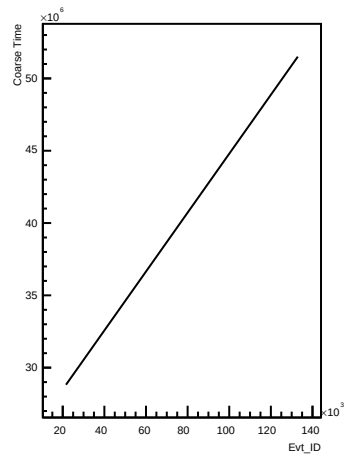
Coarse_times wrt Evt_ID for channel 229 (ping)
