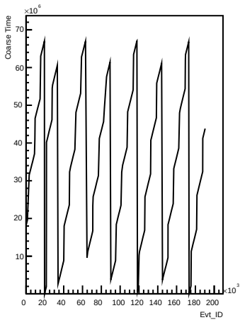
Coarse_times wrt Evt_ID for channel 113 (ping)
