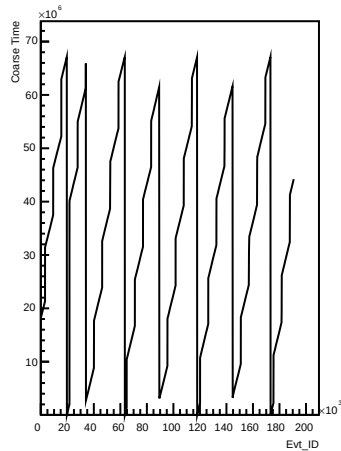
Coarse_times wrt Evt_ID for channel 98 (ping)
