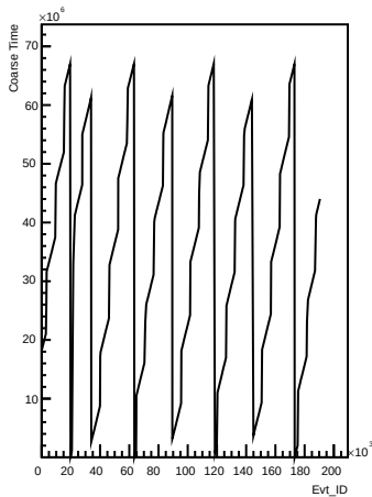
Coarse_times wrt Evt_ID for channel 33 (ping)
