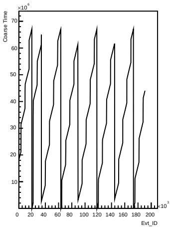
Coarse_times wrt Evt_ID for channel 40 (ping)
