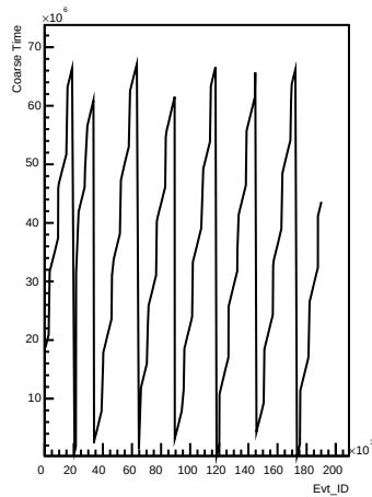
Coarse_times wrt Evt_ID for channel 126 (ping)
