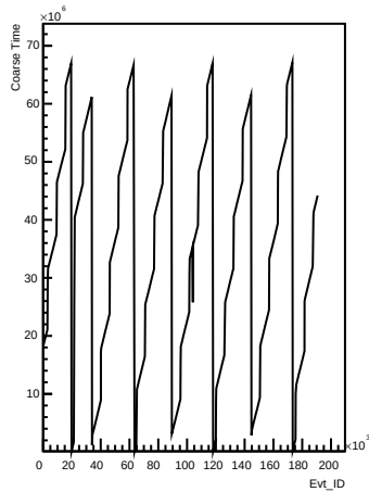
Coarse_times wrt Evt_ID for channel 95 (ping)
