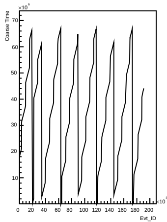
Coarse_times wrt Evt_ID for channel 114 (ping)
