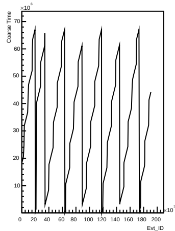
Coarse_times wrt Evt_ID for channel 103 (ping)
