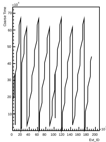
Coarse_times wrt Evt_ID for channel 26 (ping)
