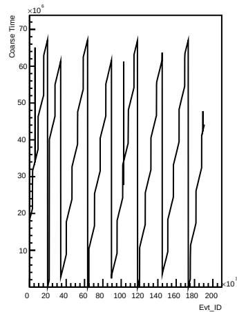
Coarse_times wrt Evt_ID for channel 19 (ping)
