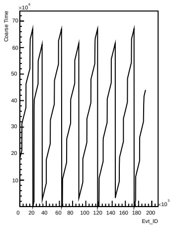
Coarse_times wrt Evt_ID for channel 104 (ping)
