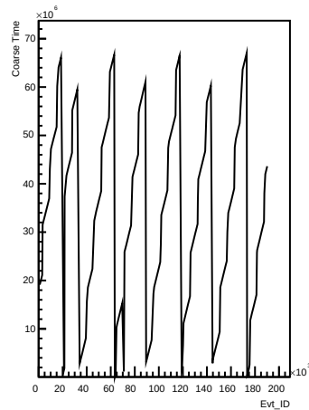
Coarse_times wrt Evt_ID for channel 111 (ping)
