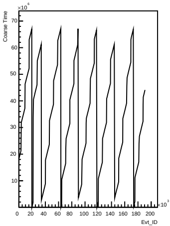
Coarse_times wrt Evt_ID for channel 44 (ping)
