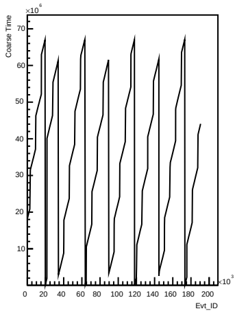
Coarse_times wrt Evt_ID for channel 84 (ping)
