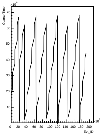
Coarse_times wrt Evt_ID for channel 5 (ping)
