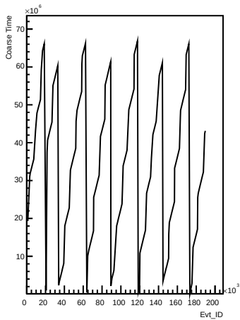
Coarse_times wrt Evt_ID for channel 105 (ping)
