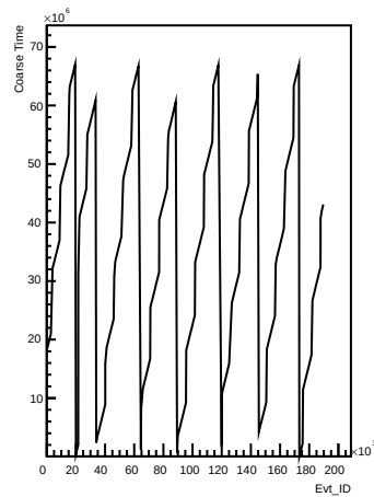
Coarse_times wrt Evt_ID for channel 123 (ping)
