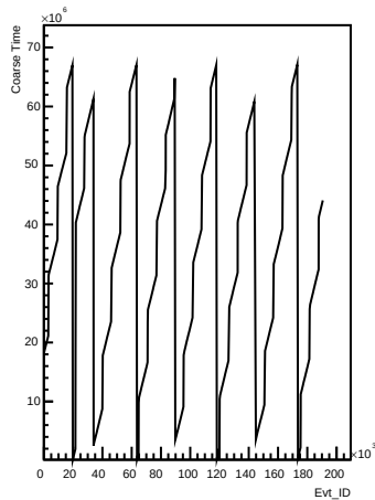
Coarse_times wrt Evt_ID for channel 118 (ping)
