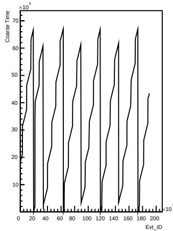
Coarse_times wrt Evt_ID for channel 55 (ping)
