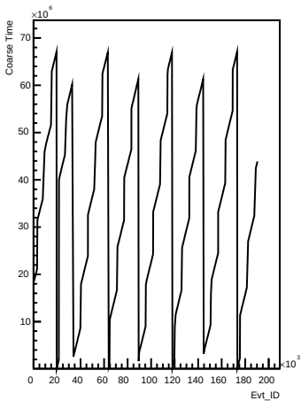
Coarse_times wrt Evt_ID for channel 76 (ping)
