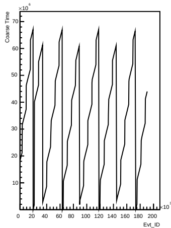
Coarse_times wrt Evt_ID for channel 79 (ping)
