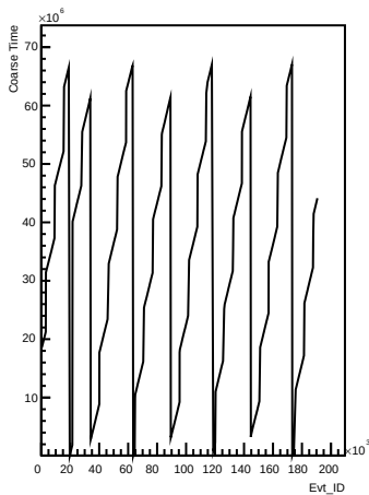
Coarse_times wrt Evt_ID for channel 74 (ping)
