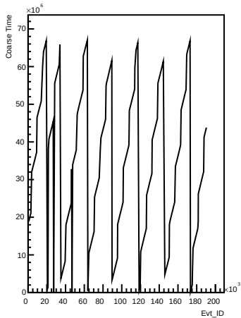
Coarse_times wrt Evt_ID for channel 96 (ping)
