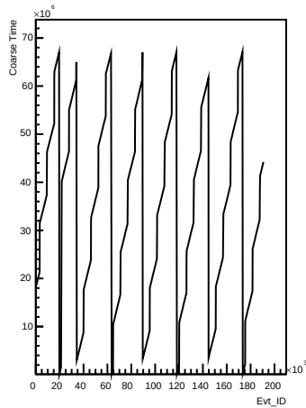
Coarse_times wrt Evt_ID for channel 46 (ping)
