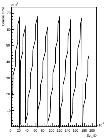
Coarse_times wrt Evt_ID for channel 120 (ping)
