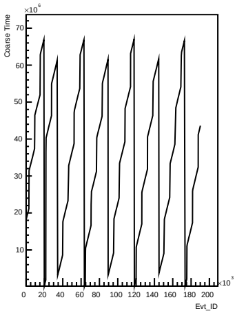
Coarse_times wrt Evt_ID for channel 56 (ping)
