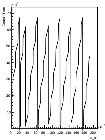
Coarse_times wrt Evt_ID for channel 109 (ping)
