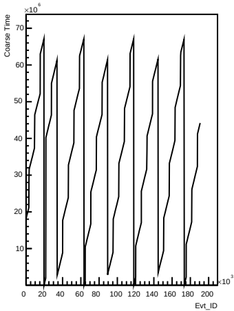
Coarse_times wrt Evt_ID for channel 68 (ping)
