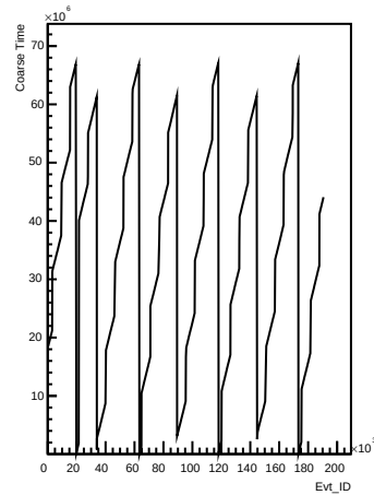
Coarse_times wrt Evt_ID for channel 87 (ping)
