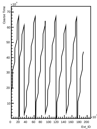
Coarse_times wrt Evt_ID for channel 3 (ping)
