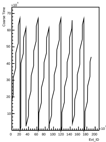
Coarse_times wrt Evt_ID for channel 125 (ping)
