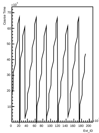
Coarse_times wrt Evt_ID for channel 122 (ping)
