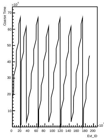
Coarse_times wrt Evt_ID for channel 34 (ping)
