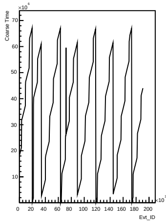
Coarse_times wrt Evt_ID for channel 6 (ping)
