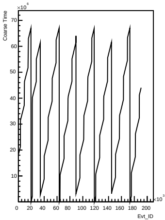
Coarse_times wrt Evt_ID for channel 4 (ping)
