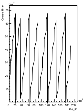
Coarse_times wrt Evt_ID for channel 24 (ping)
