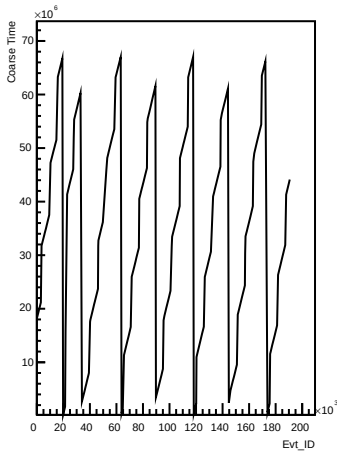
Coarse_times wrt Evt_ID for channel 65 (ping)
