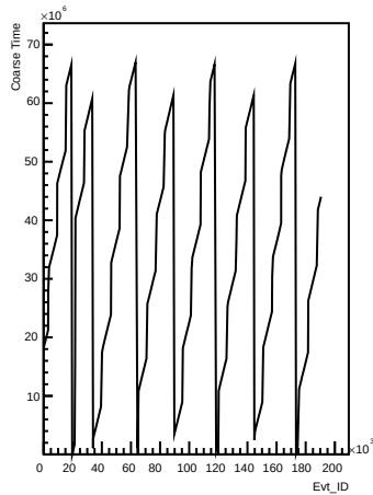
Coarse_times wrt Evt_ID for channel 67 (ping)
