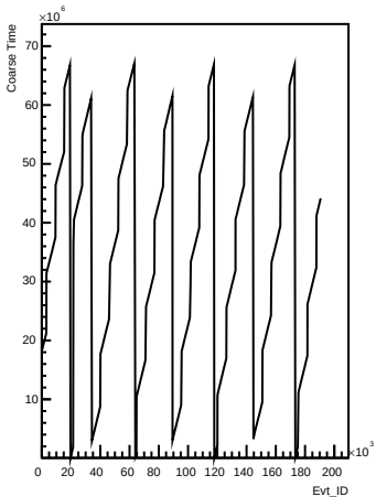
Coarse_times wrt Evt_ID for channel 60 (ping)
