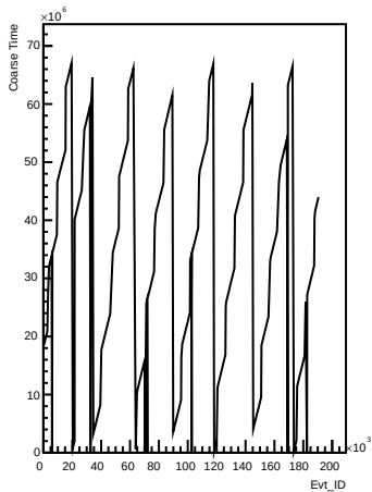
Coarse_times wrt Evt_ID for channel 16 (ping)
