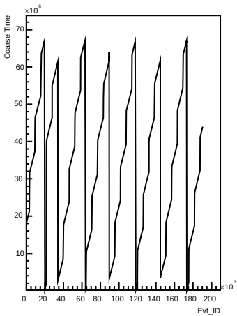
Coarse_times wrt Evt_ID for channel 0 (ping)
