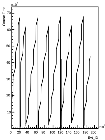
Coarse_times wrt Evt_ID for channel 1 (ping)
