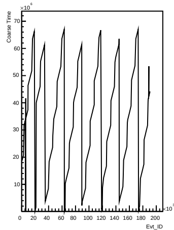
Coarse_times wrt Evt_ID for channel 23 (ping)
