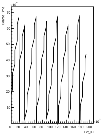
Coarse_times wrt Evt_ID for channel 116 (ping)
