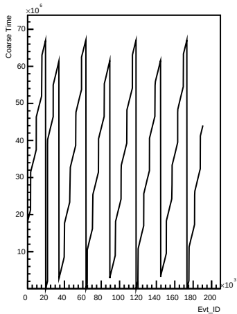
Coarse_times wrt Evt_ID for channel 12 (ping)
