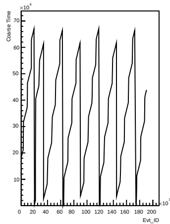
Coarse_times wrt Evt_ID for channel 115 (ping)
