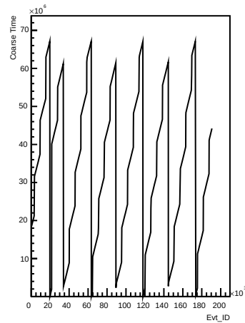
Coarse_times wrt Evt_ID for channel 83 (ping)
