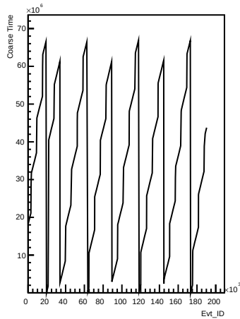
Coarse_times wrt Evt_ID for channel 66 (ping)
