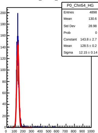
P0_Chn54_HG
