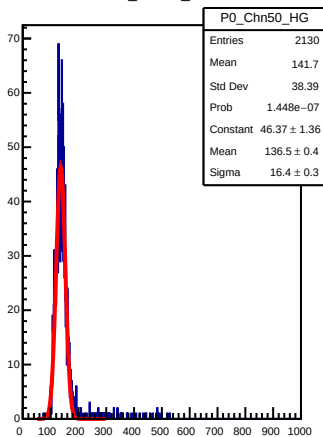
P0_Chn50_HG
