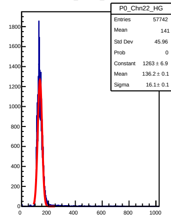
P0_Chnl22_HG
