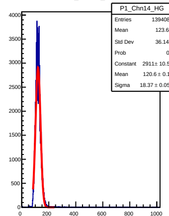
P1_Ch14_HG
