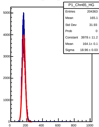
P1_Chn65_HG
