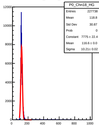
P0_Chnl8_HG
