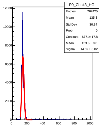
P0_Chn43_HG
