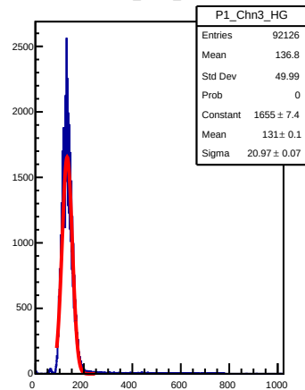
P1_Ch3n3_HG
