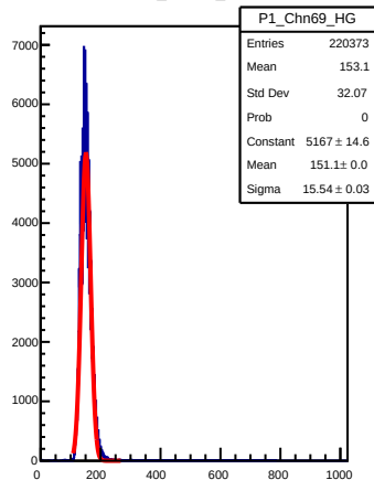
P1_Chn69_HG
