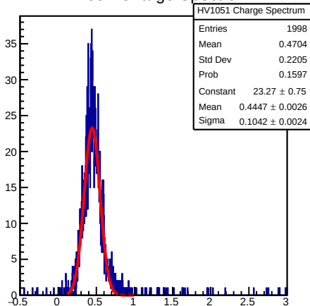
HV1051 Charge Spectrum
