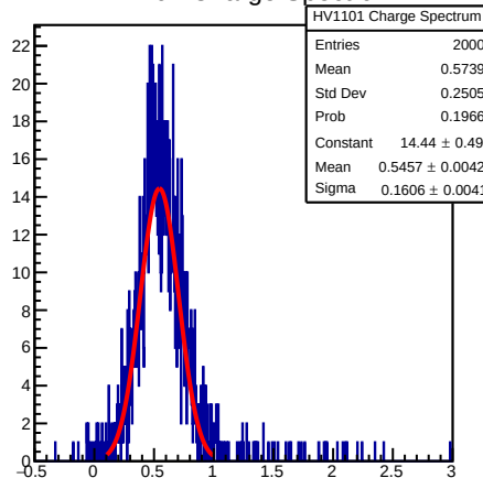
HV1101 Charge Spectrum
