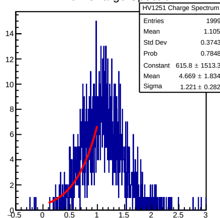
HV1251 Charge Spectrum
