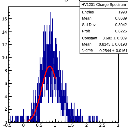
HV1201 Charge Spectrum
