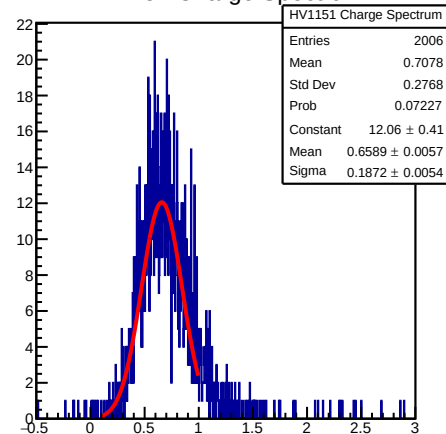
HV1151 Charge Spectrum
