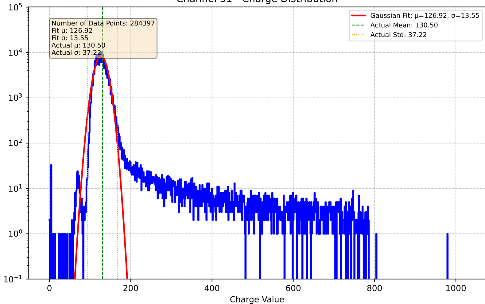
Channel 51 - Charge Distribution
