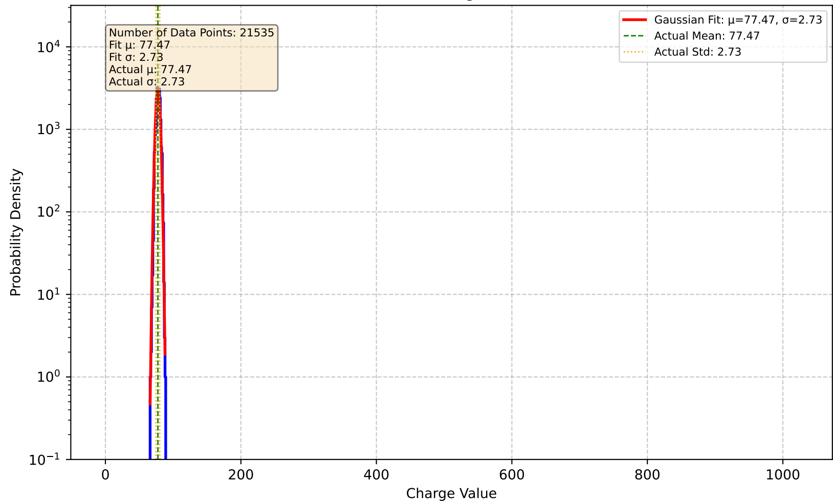
Channel 10 - Charge Distribution
