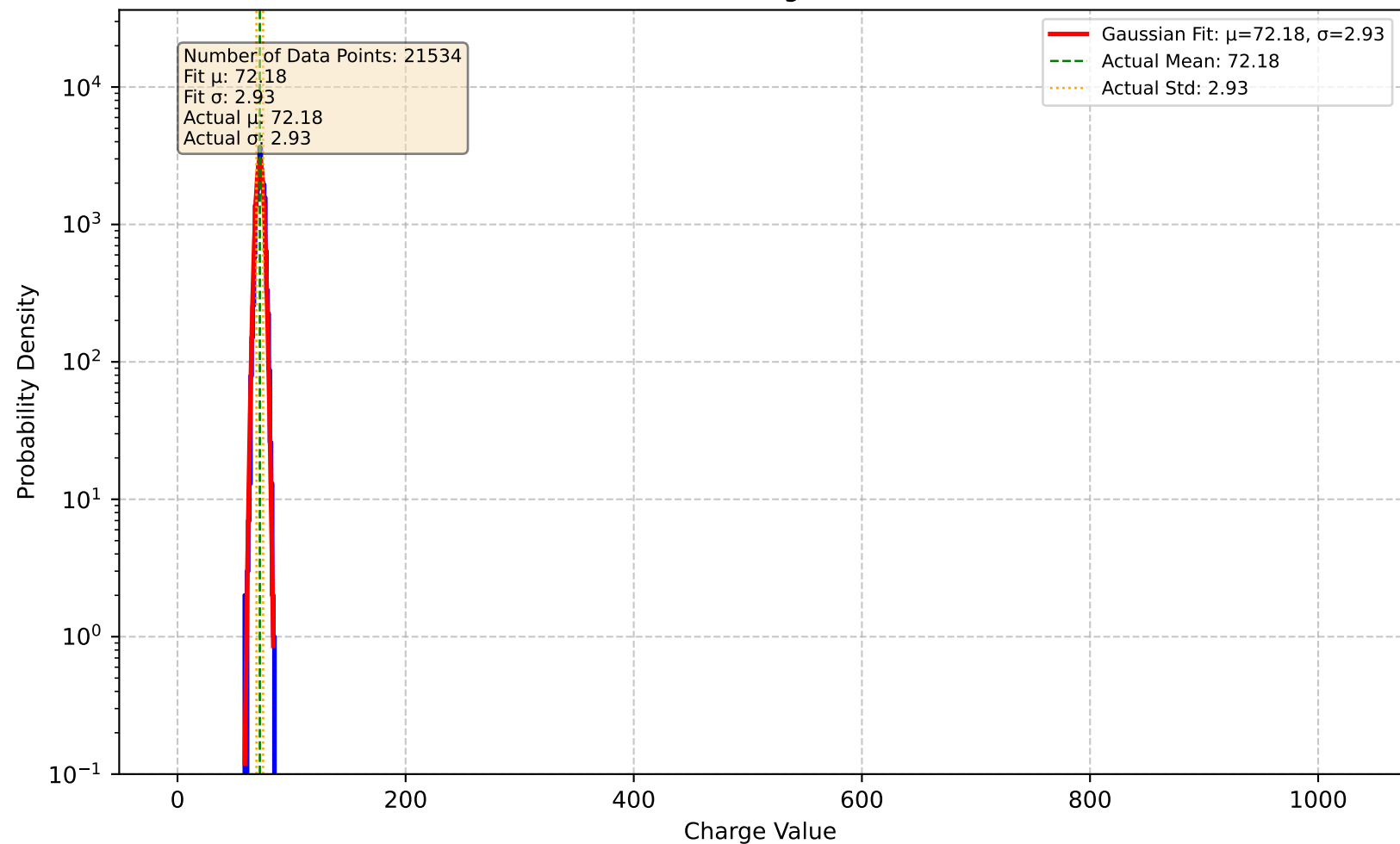
Channel 99 - Charge Distribution
