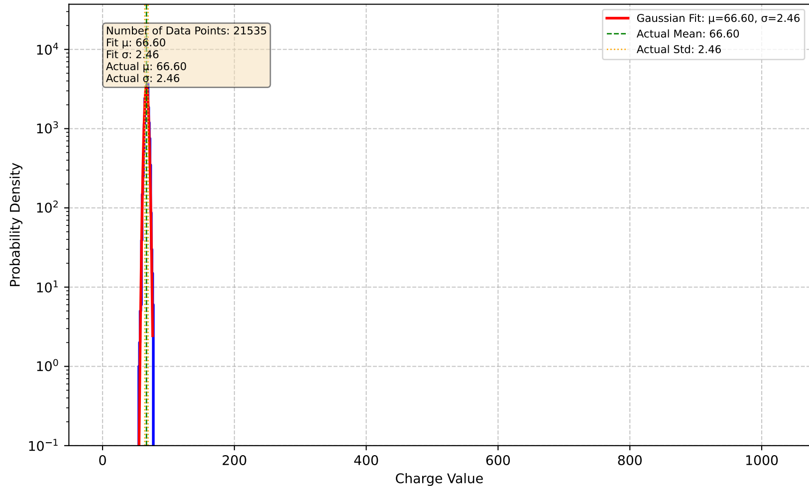
Channel 47 - Charge Distribution
