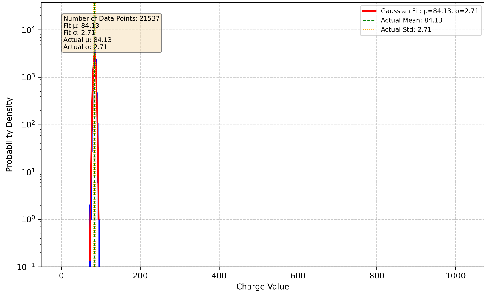
Channel 70 - Charge Distribution
