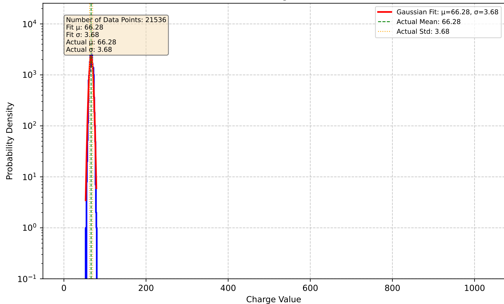
Channel 37 - Charge Distribution
