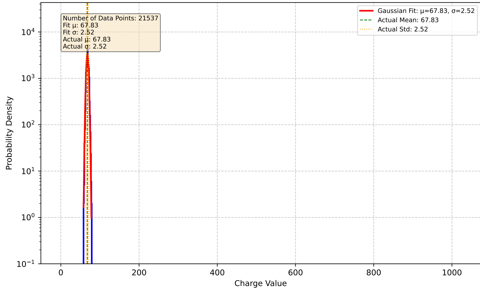
Channel 93 - Charge Distribution
