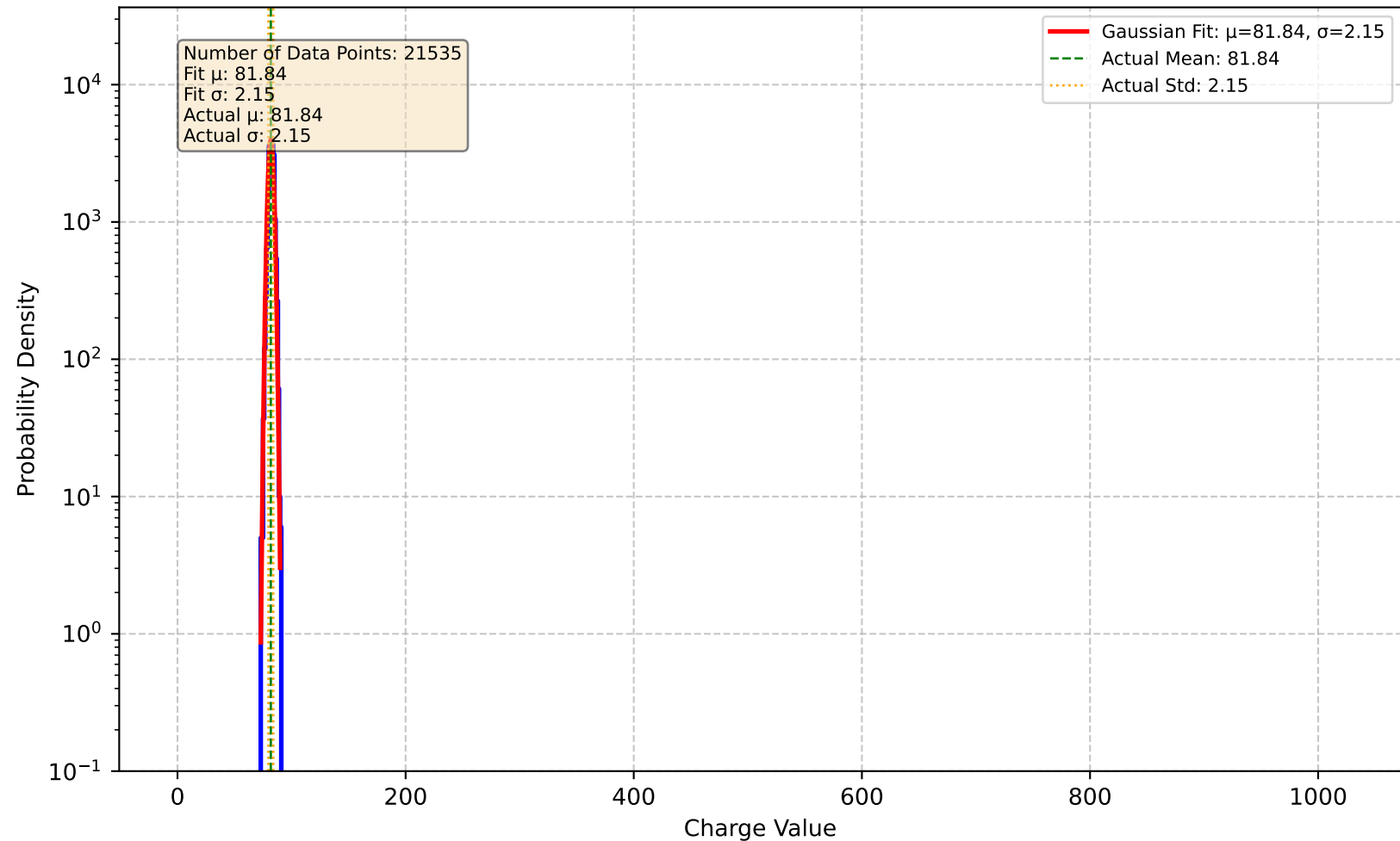
Channel 73 - Charge Distribution
