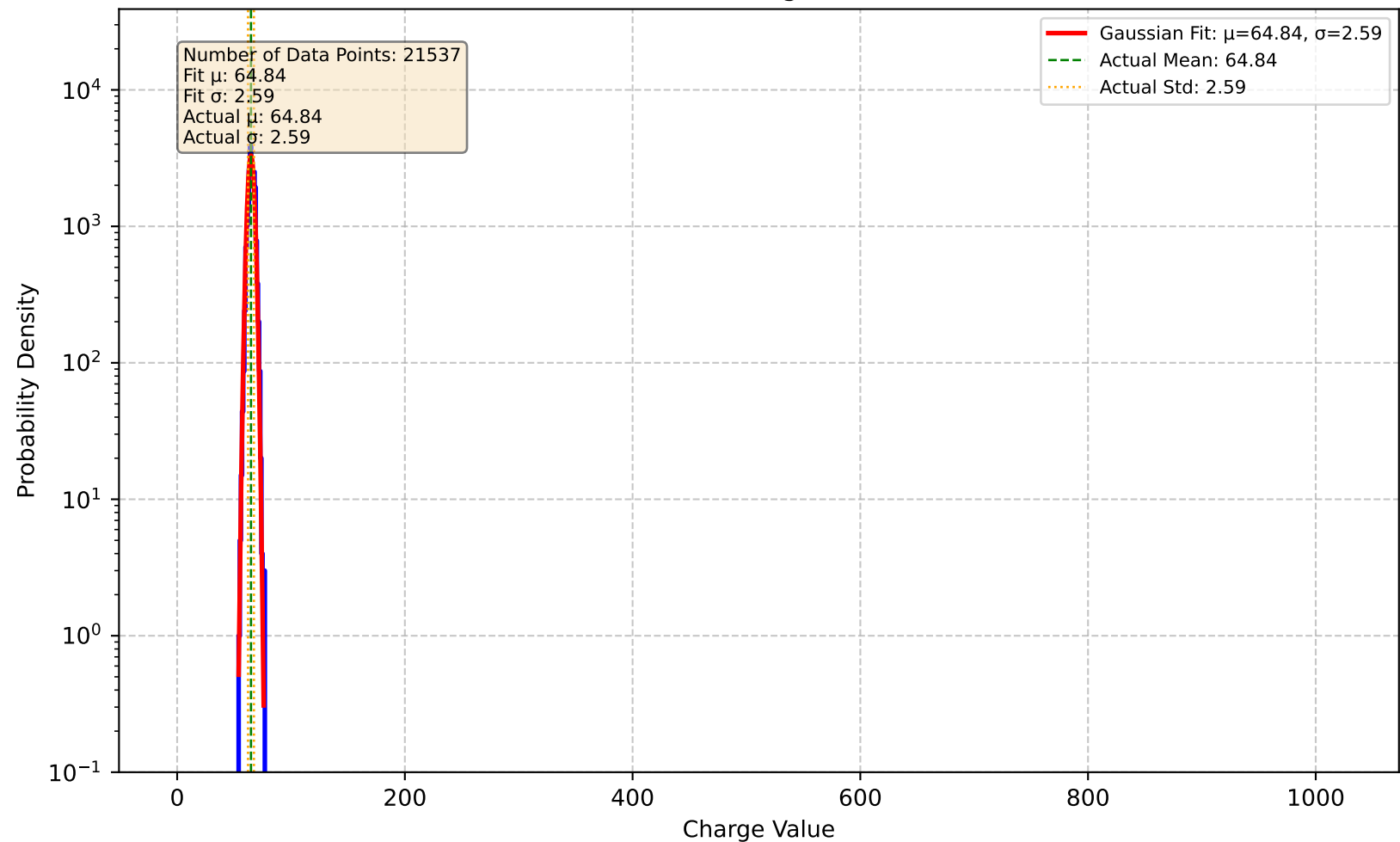
Channel 44 - Charge Distribution
