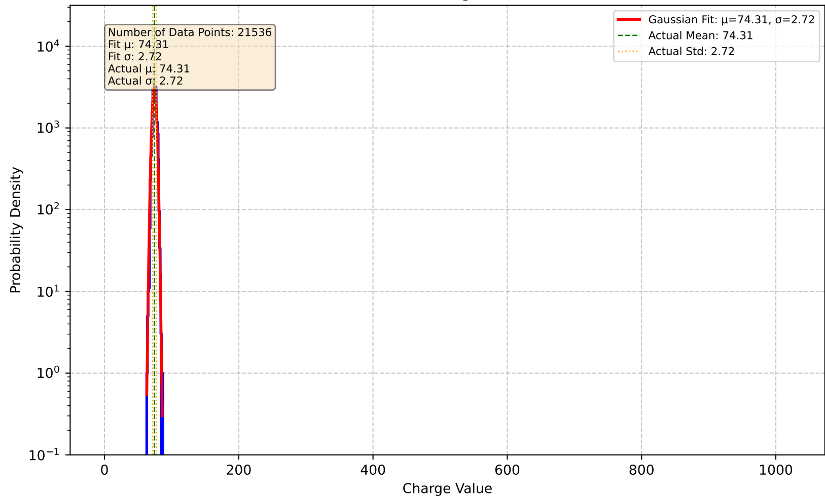
Channel 48 - Charge Distribution
