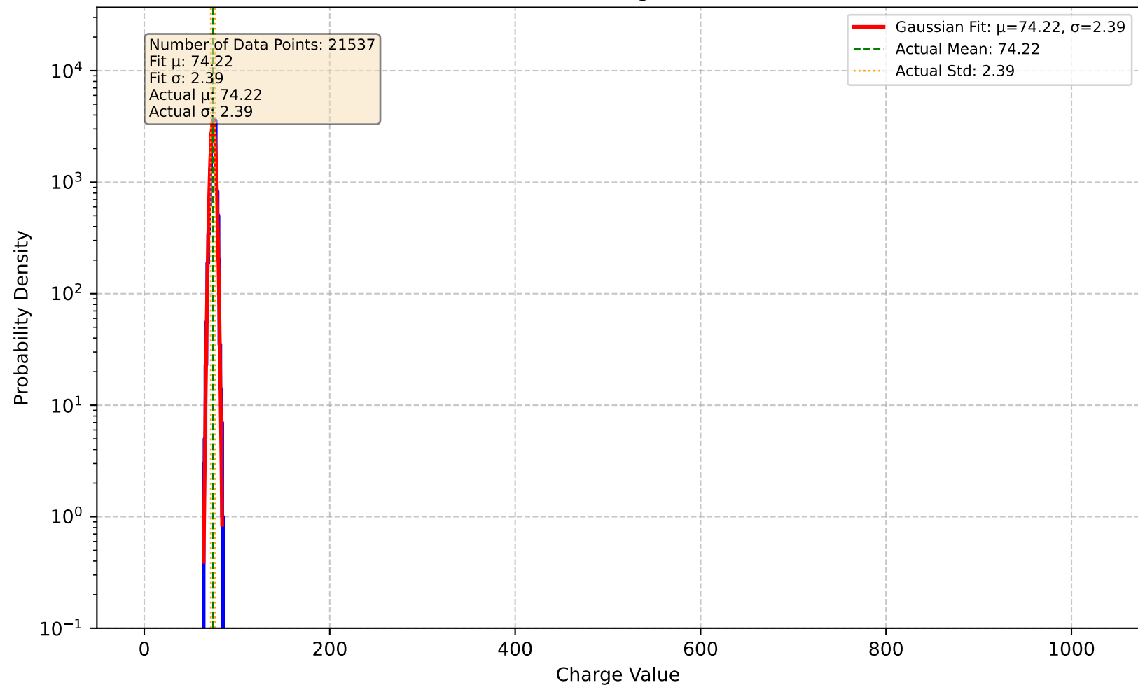
Channel 62 - Charge Distribution
