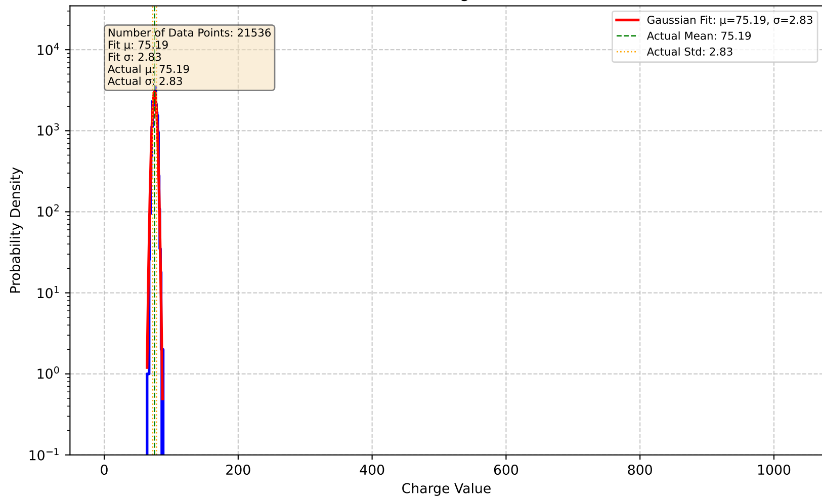
Channel 55 - Charge Distribution
