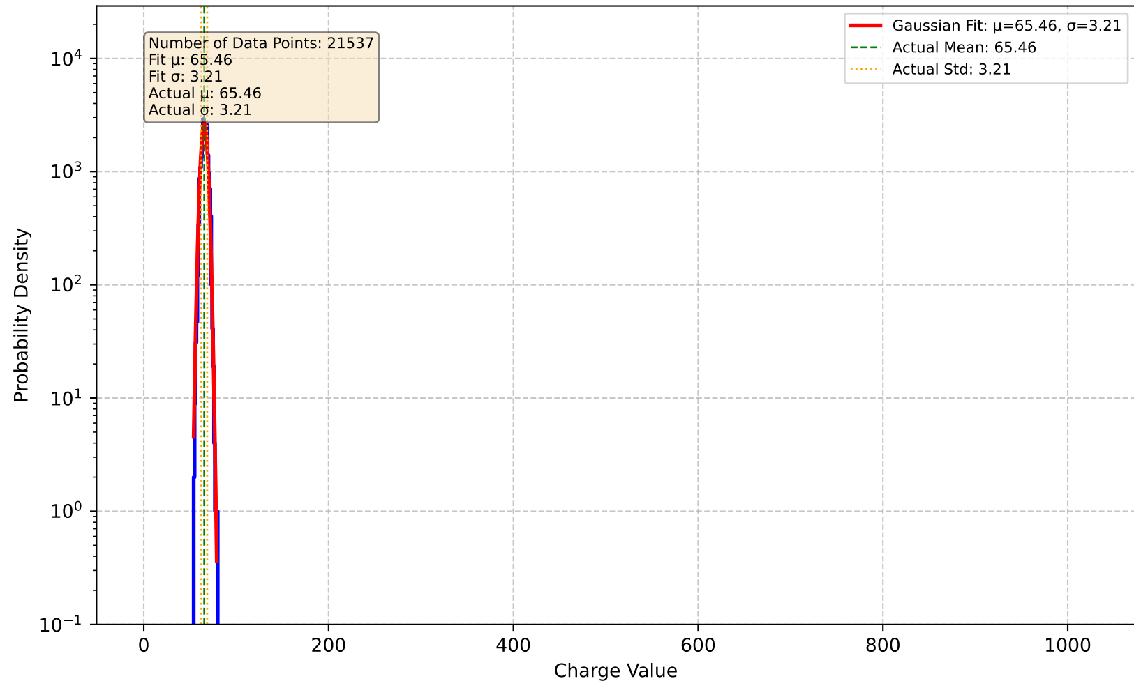
Channel 36 - Charge Distribution
