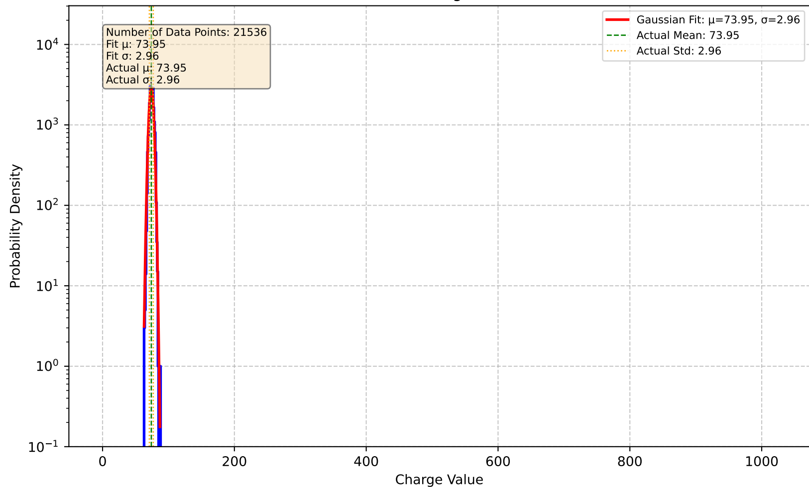
Channel 59 - Charge Distribution
