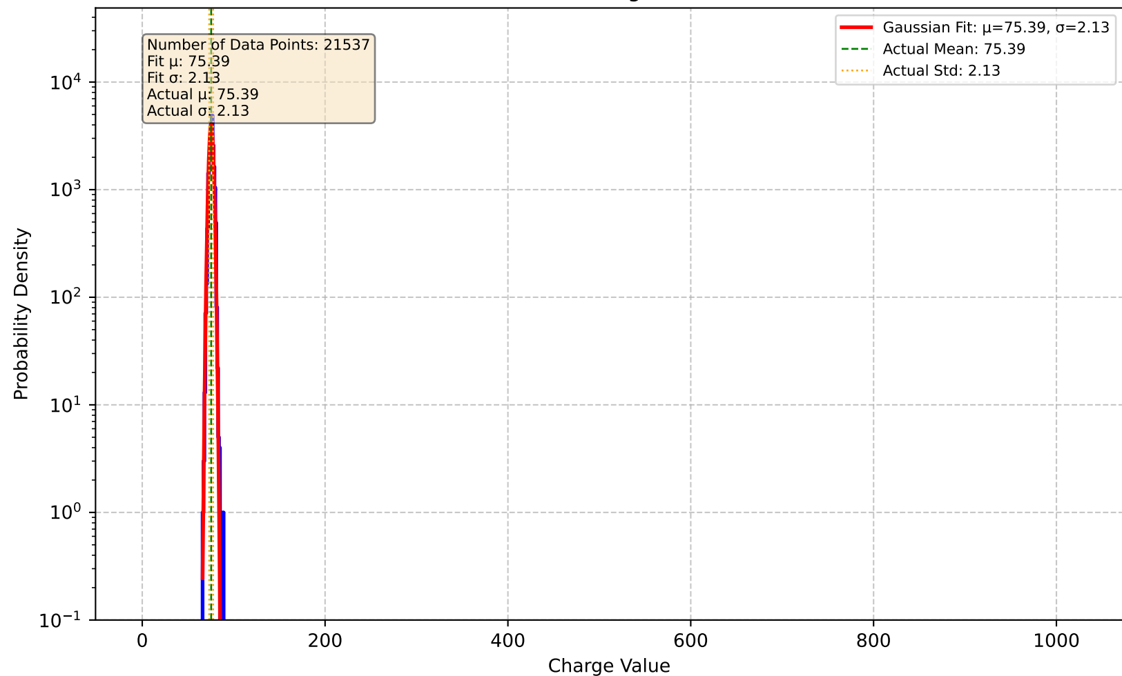
Channel 56 - Charge Distribution
