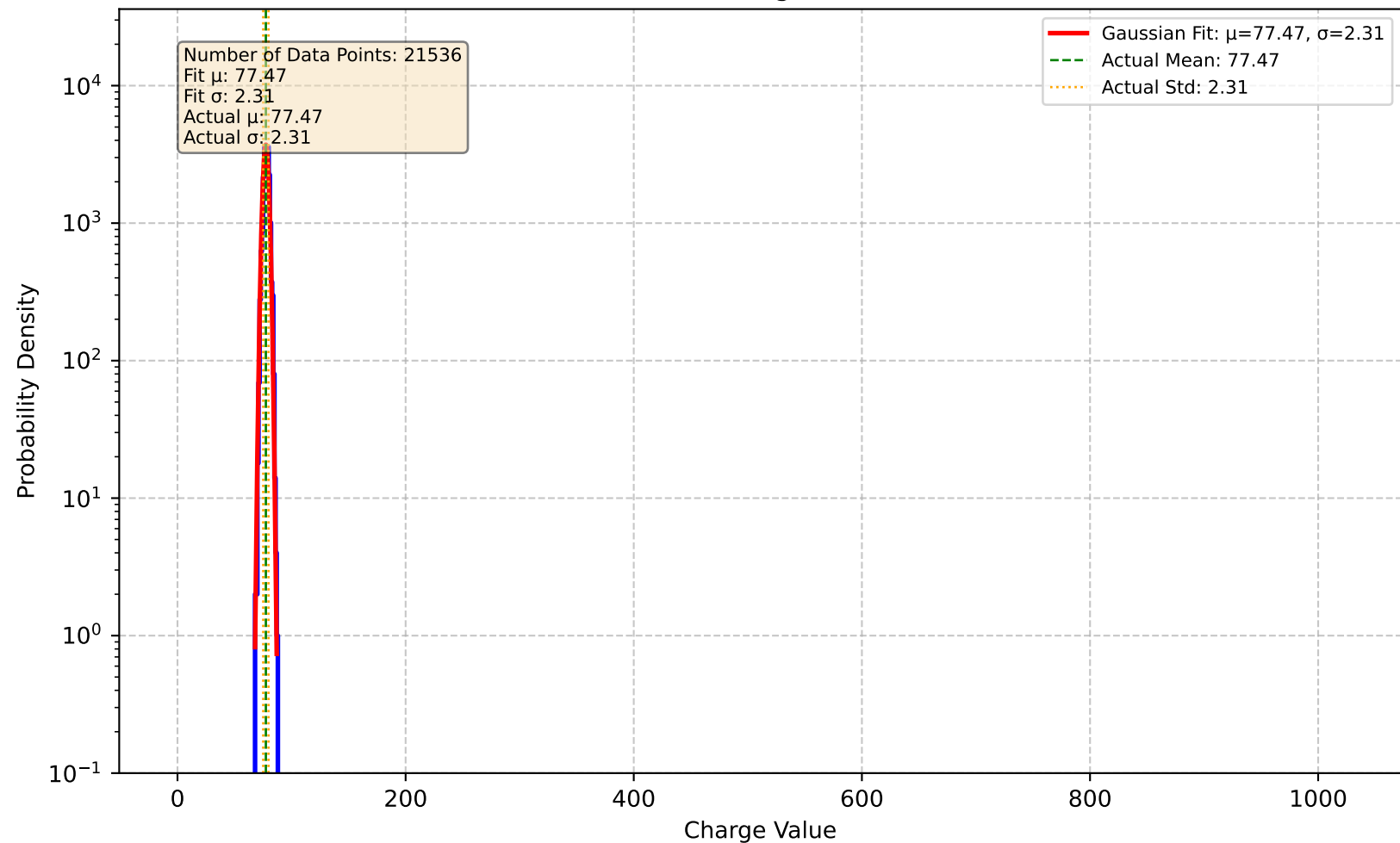
Channel 7 - Charge Distribution
