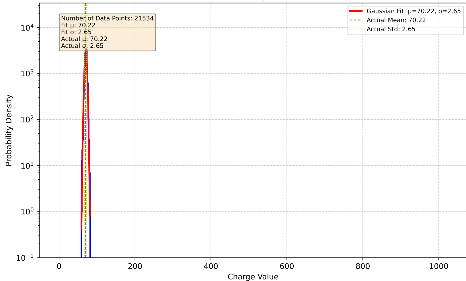
Channel 84 - Charge Distribution
