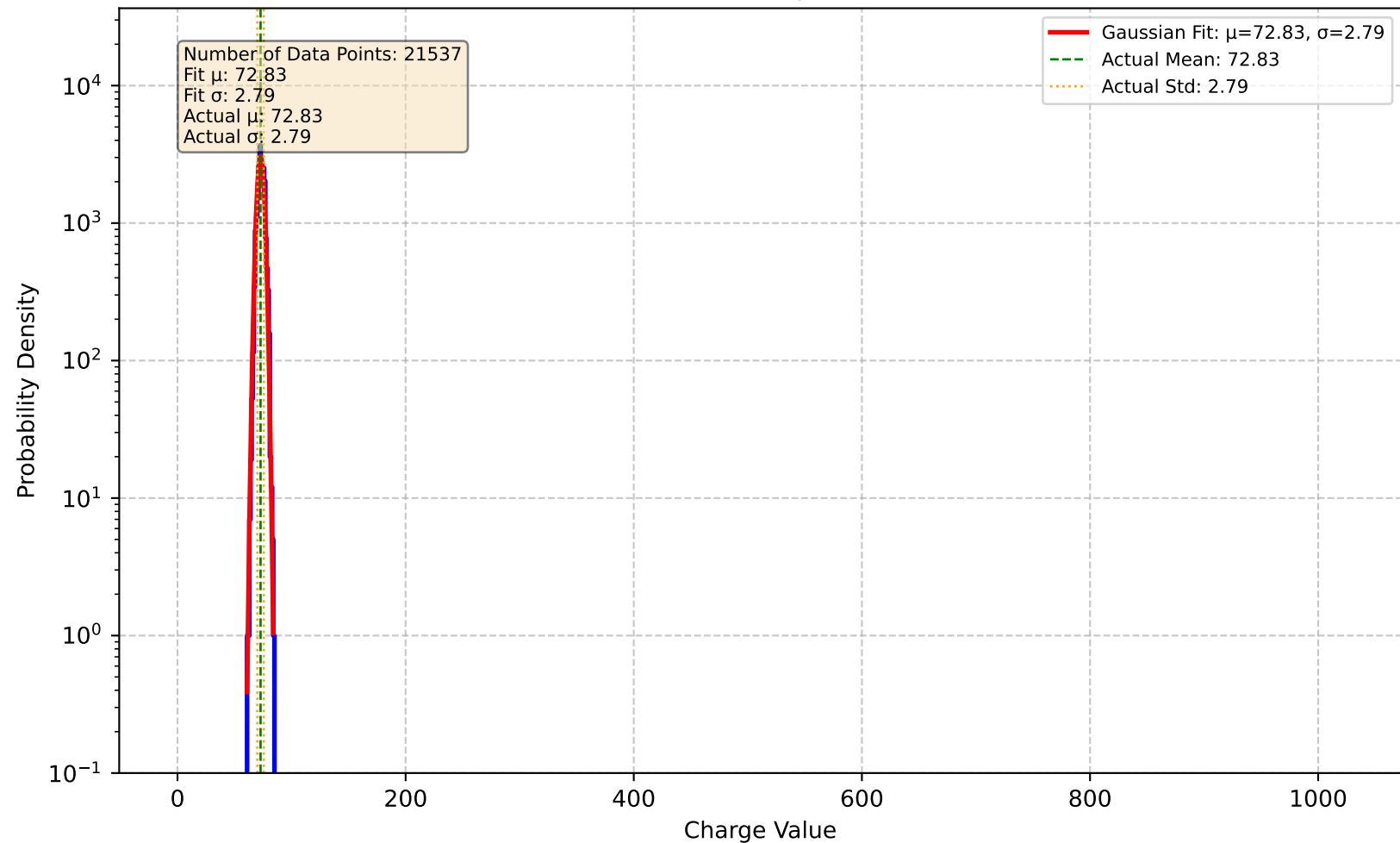
Channel 107 - Charge Distribution
