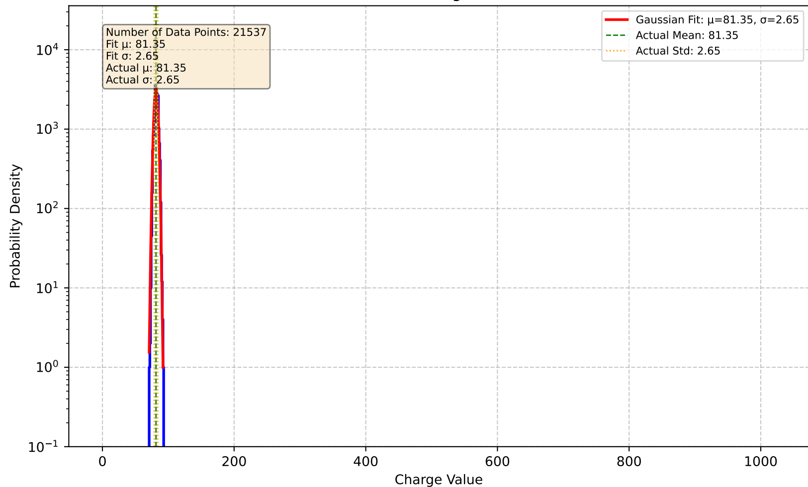
Channel 76 - Charge Distribution
