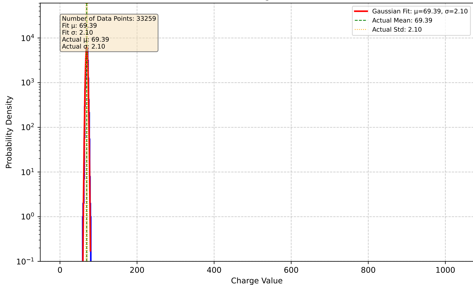
Channel 97 - Charge Distribution
