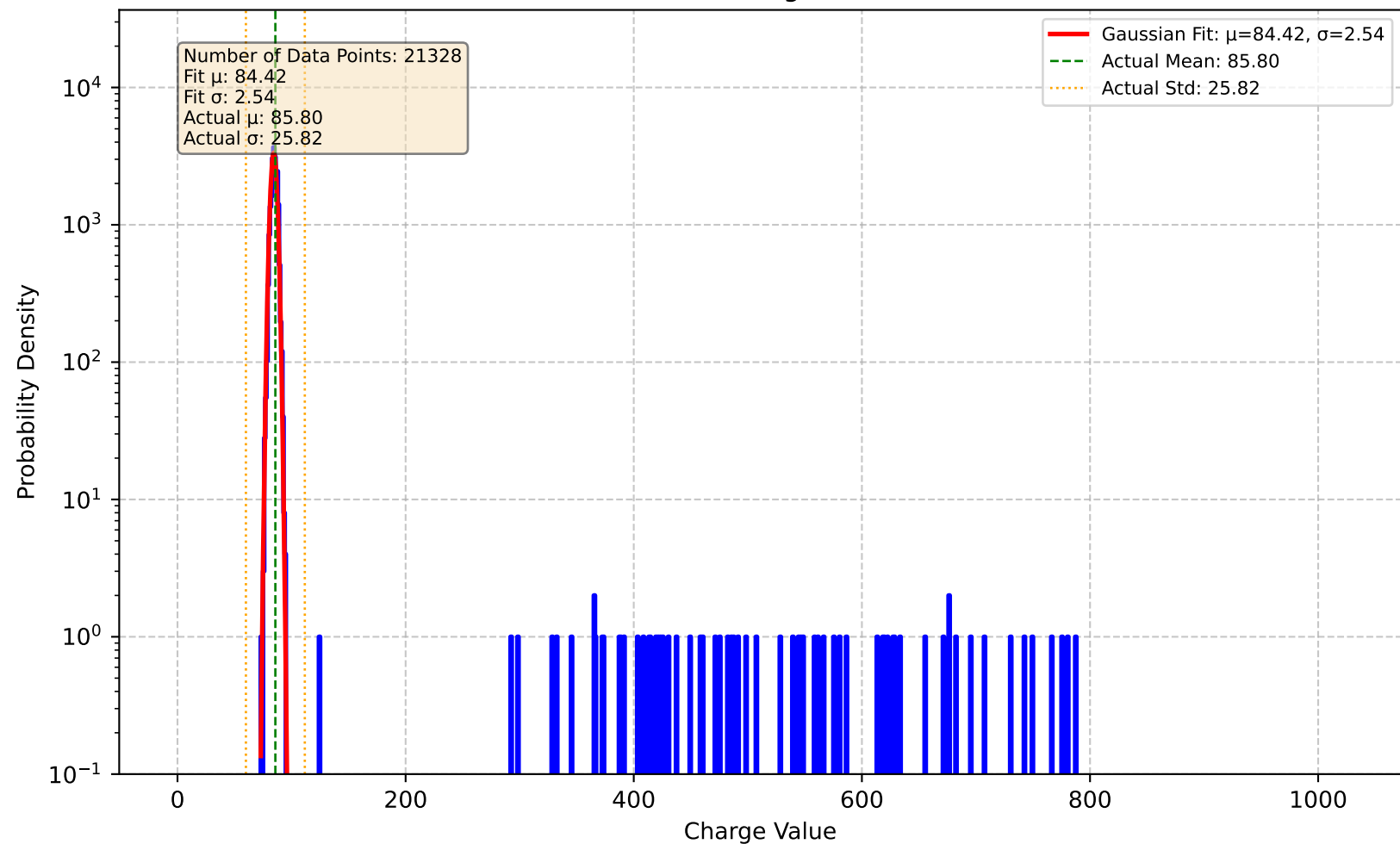
Channel 88 - Charge Distribution
