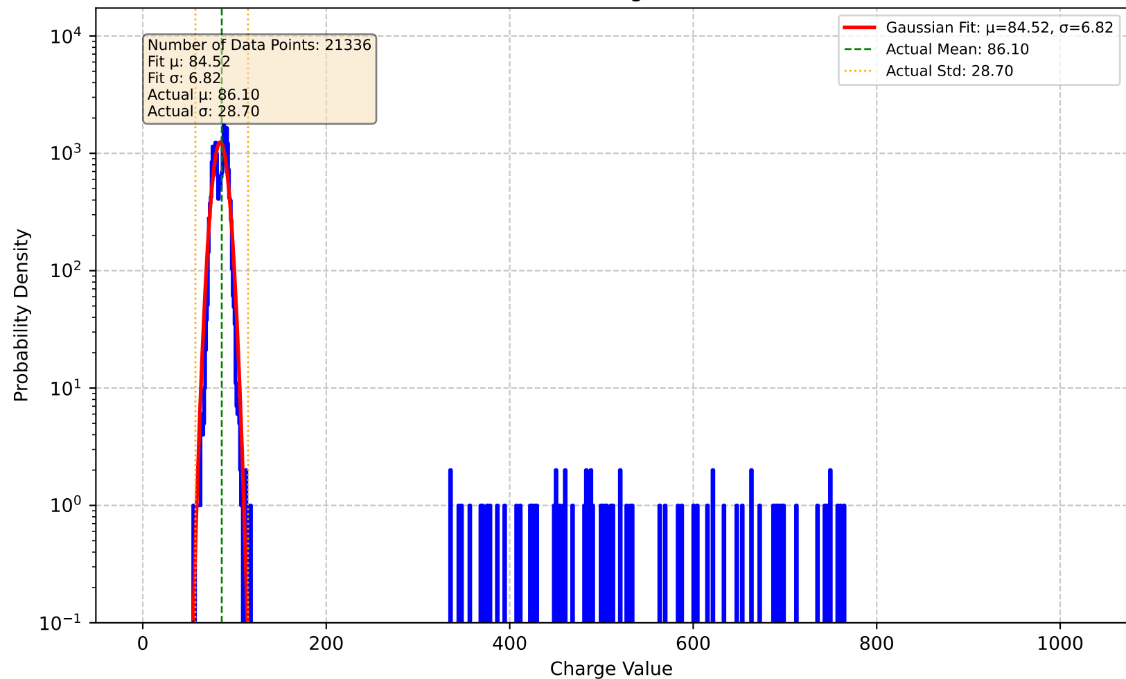
Channel 57 - Charge Distribution
