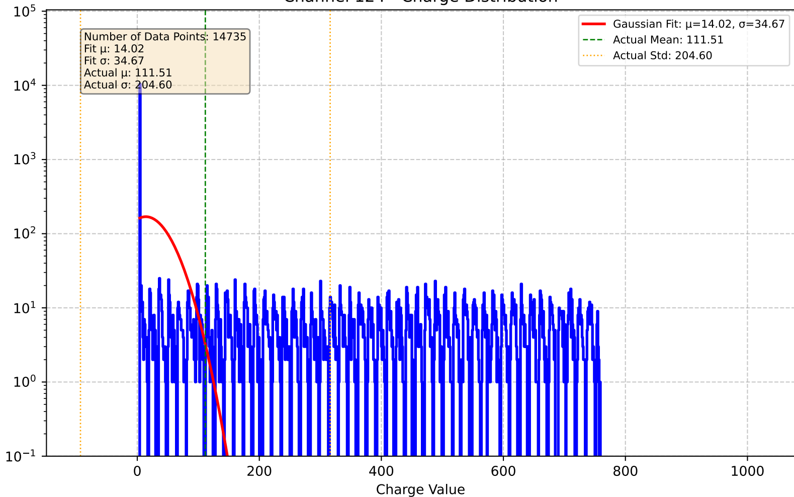
Channel 124 - Charge Distribution
