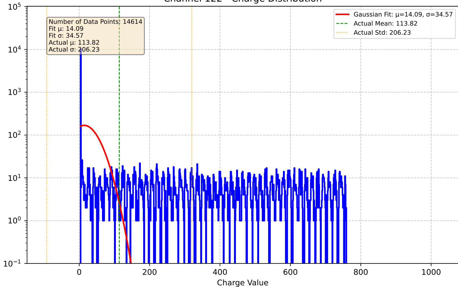
Channel 122 - Charge Distribution
