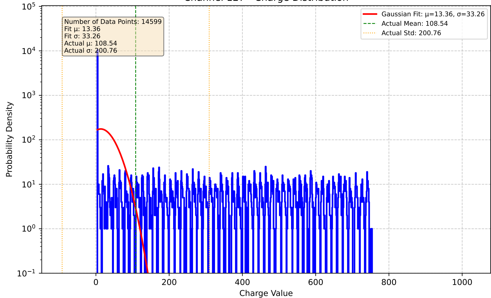
Channel 127 - Charge Distribution
