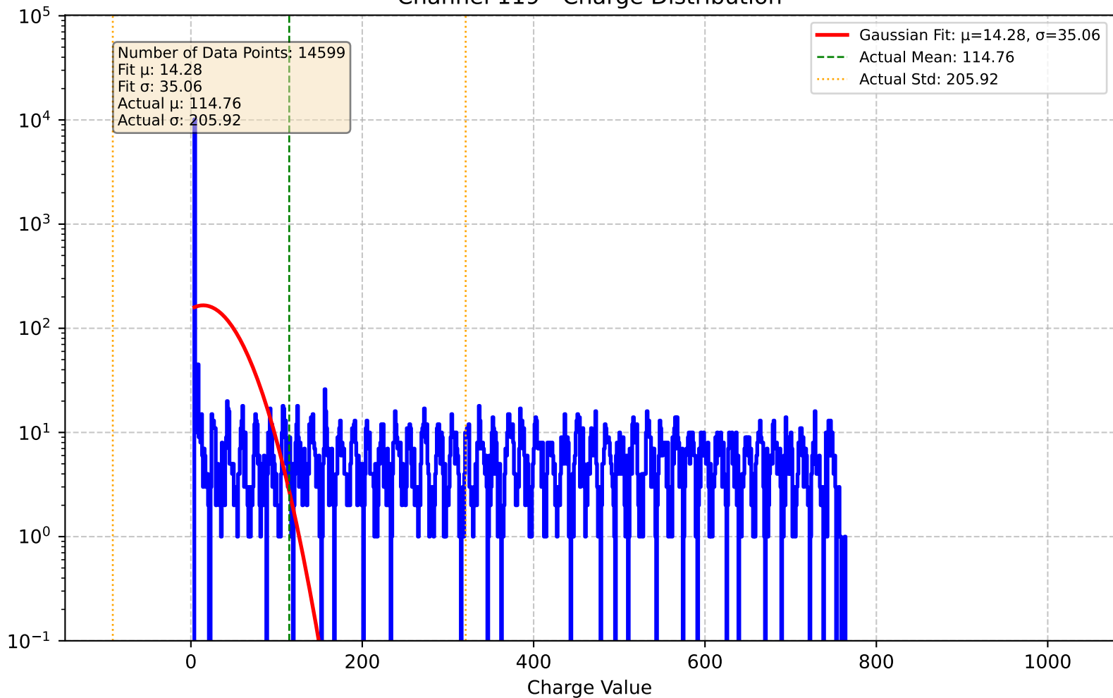
Channel 119 - Charge Distribution
