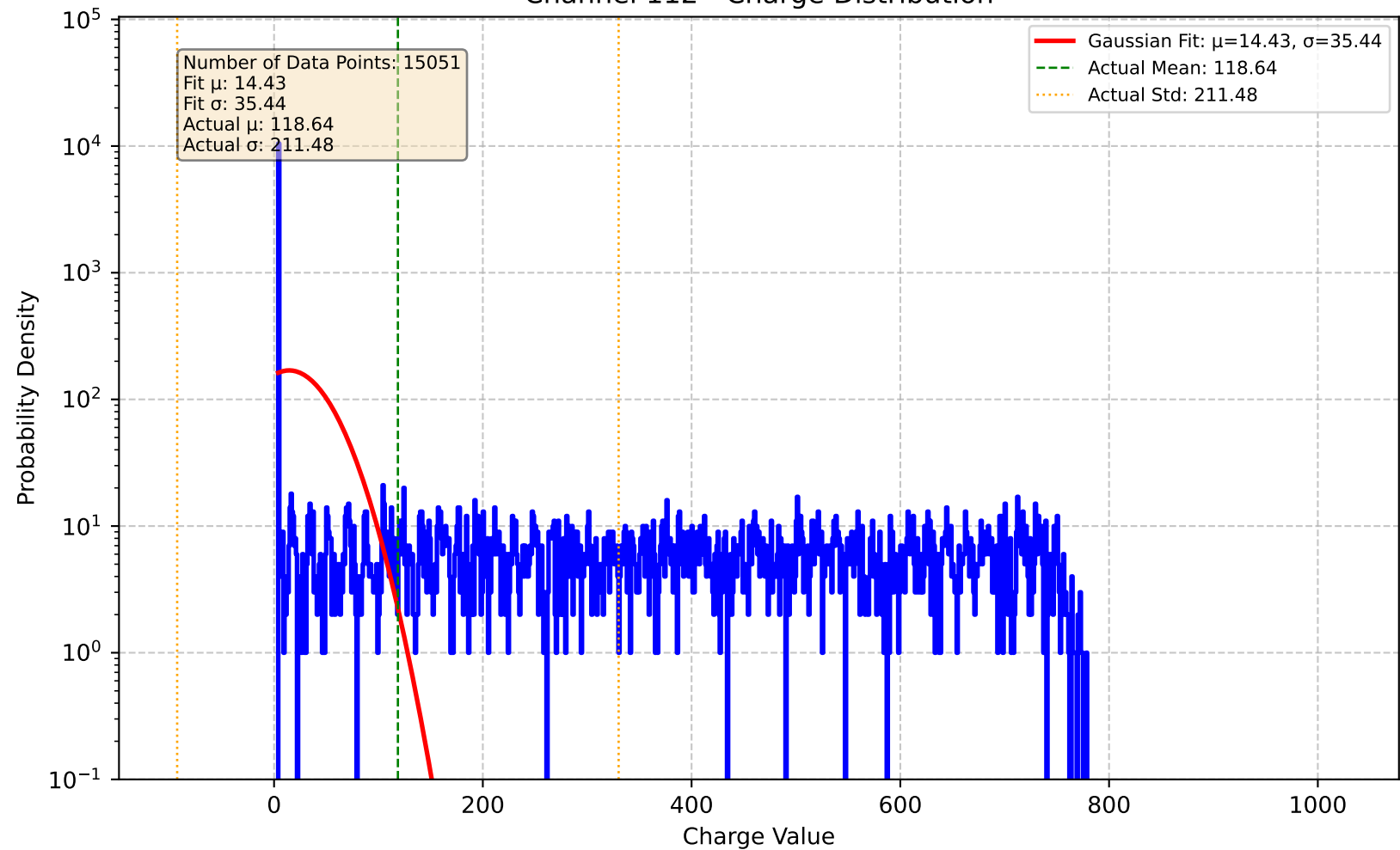
Channel 112 - Charge Distribution
