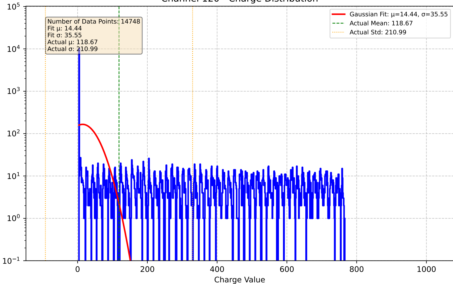
Channel 120 - Charge Distribution
