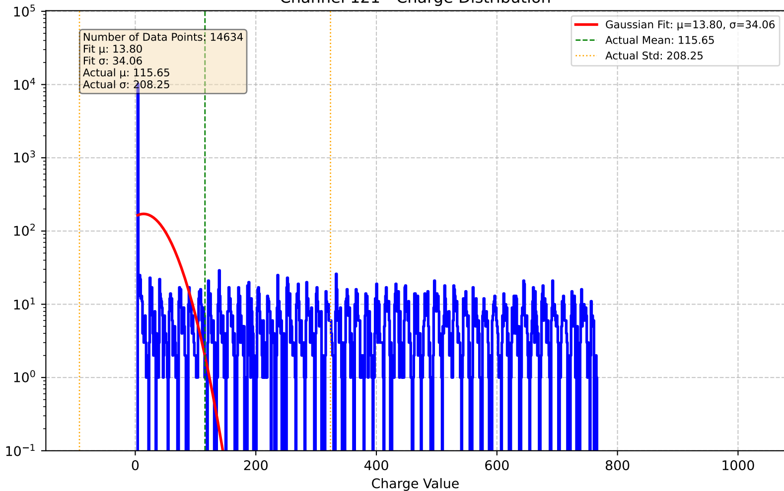
Channel 121 - Charge Distribution
