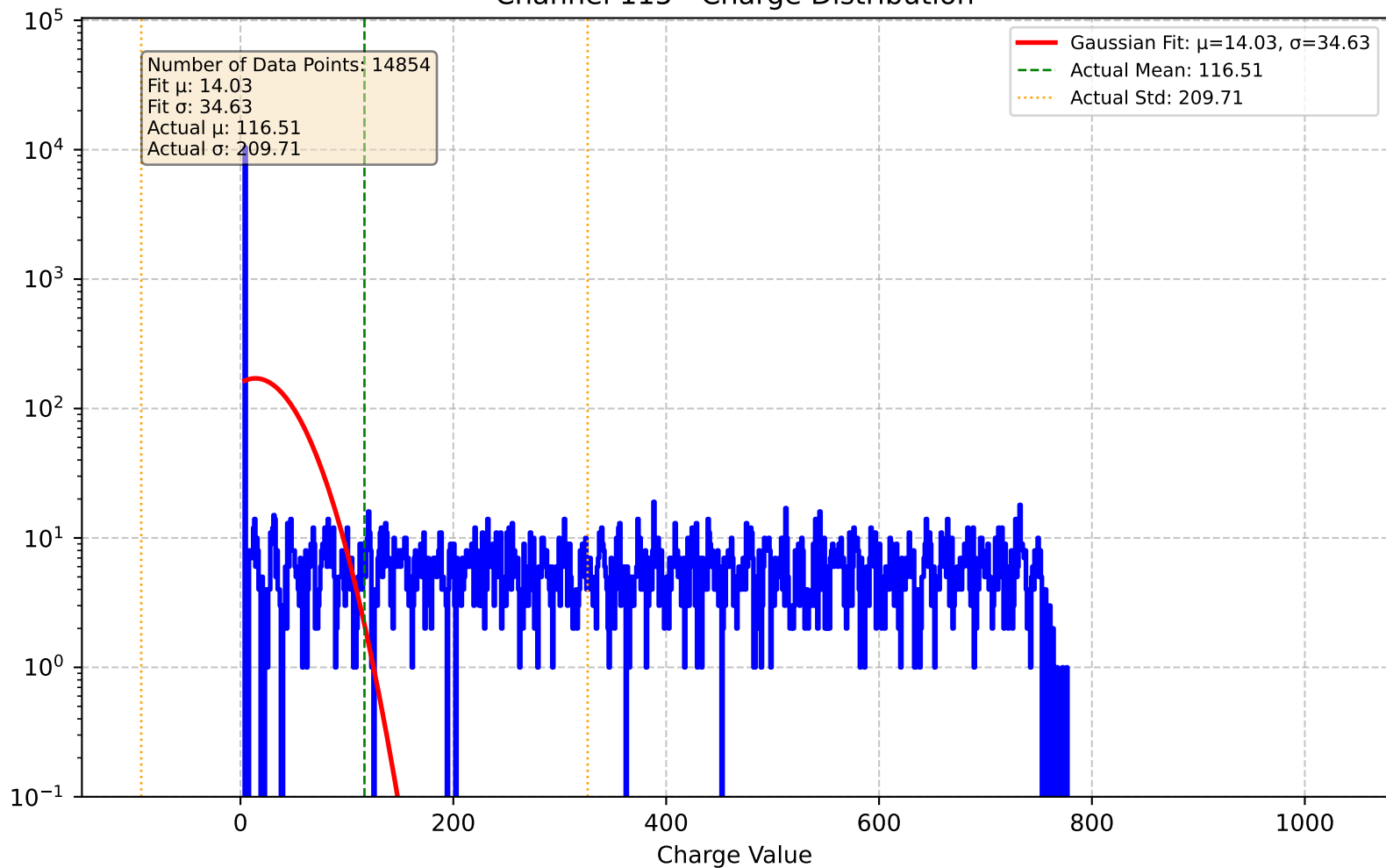
Channel 115 - Charge Distribution
