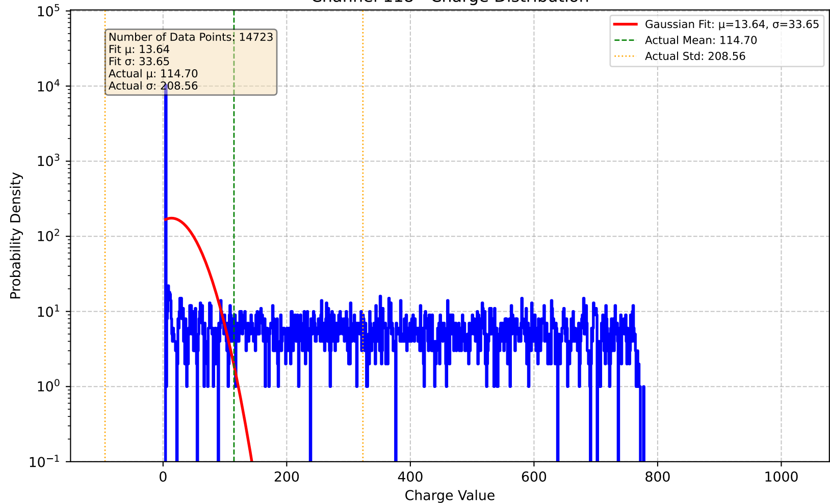
Channel 118 - Charge Distribution
