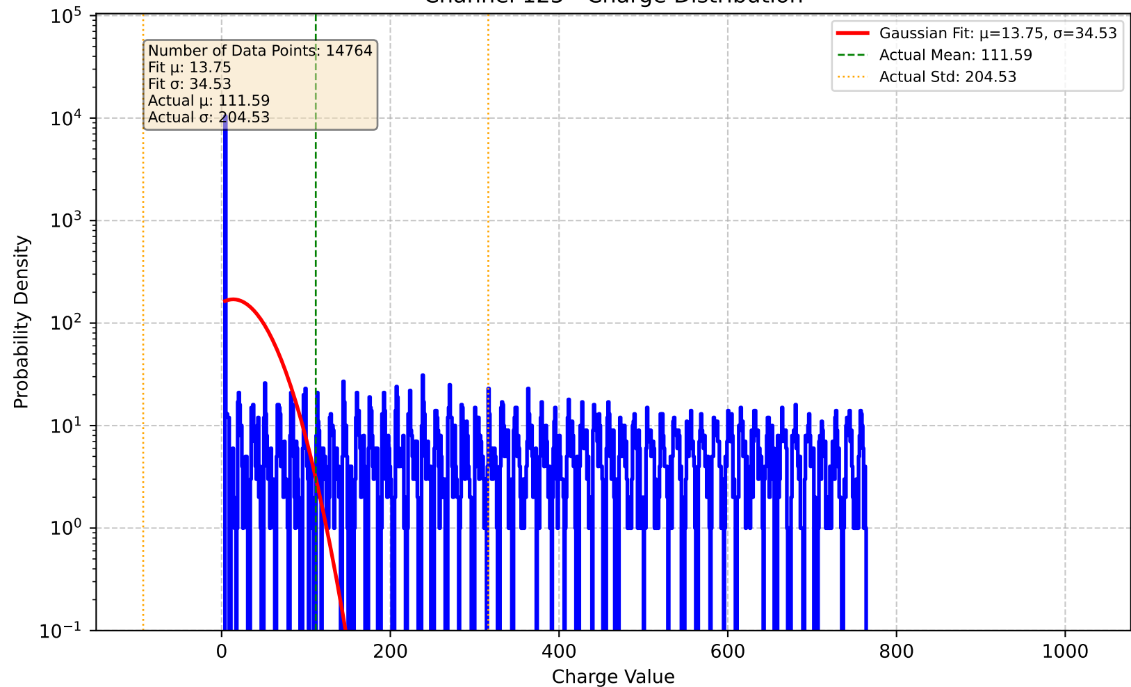
Channel 125 - Charge Distribution
