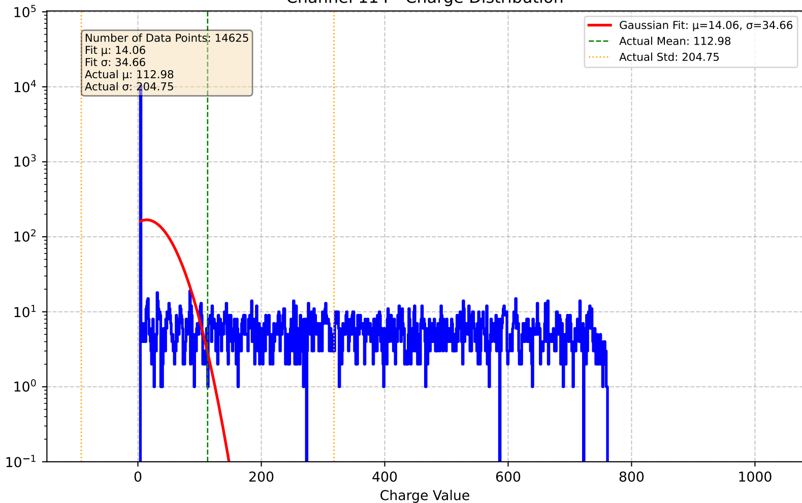
Channel 114 - Charge Distribution
