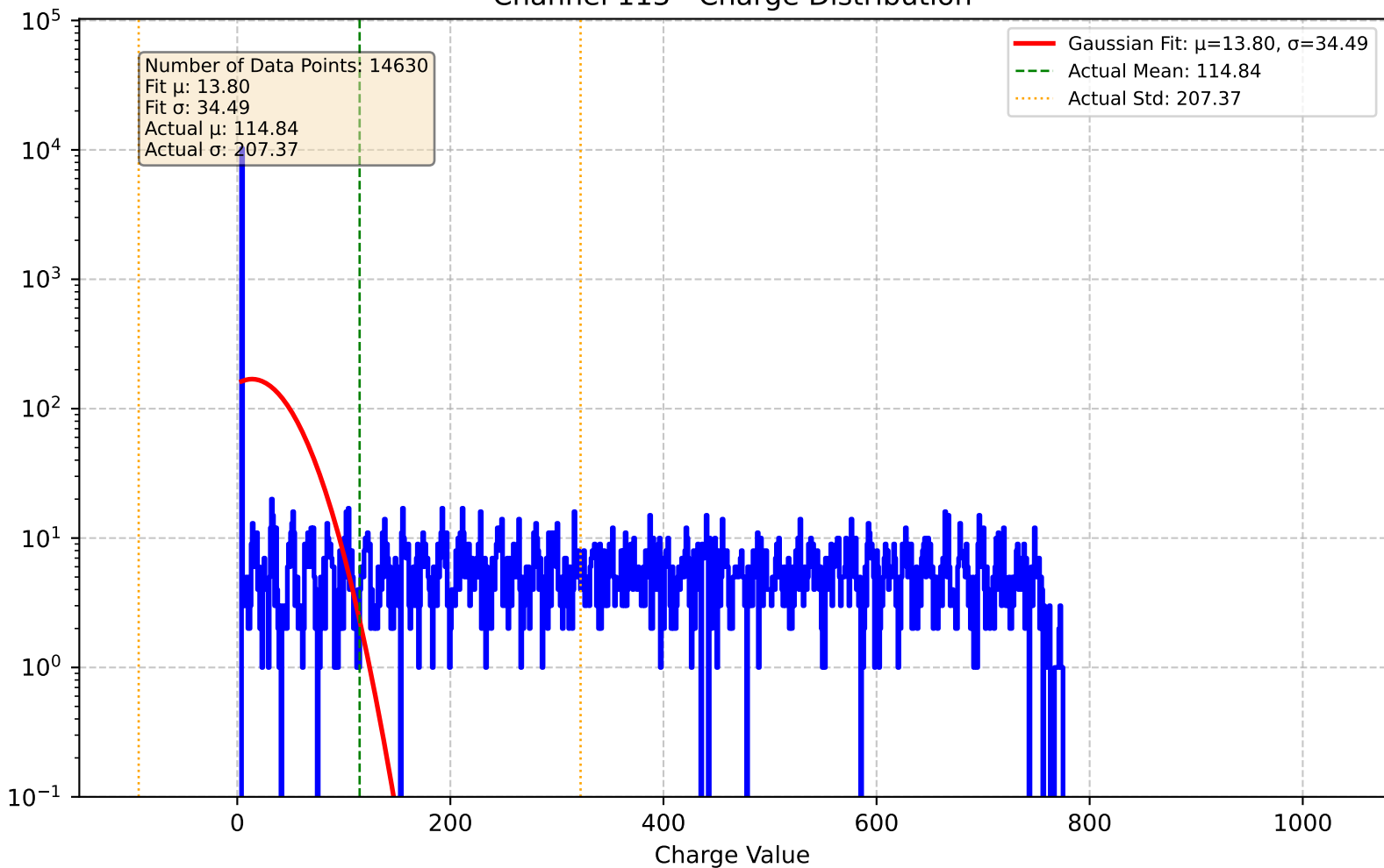
Channel 113 - Charge Distribution
