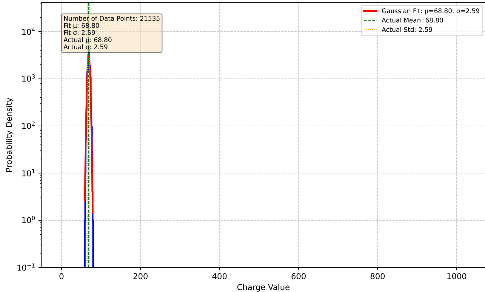
Channel 45 - Charge Distribution
