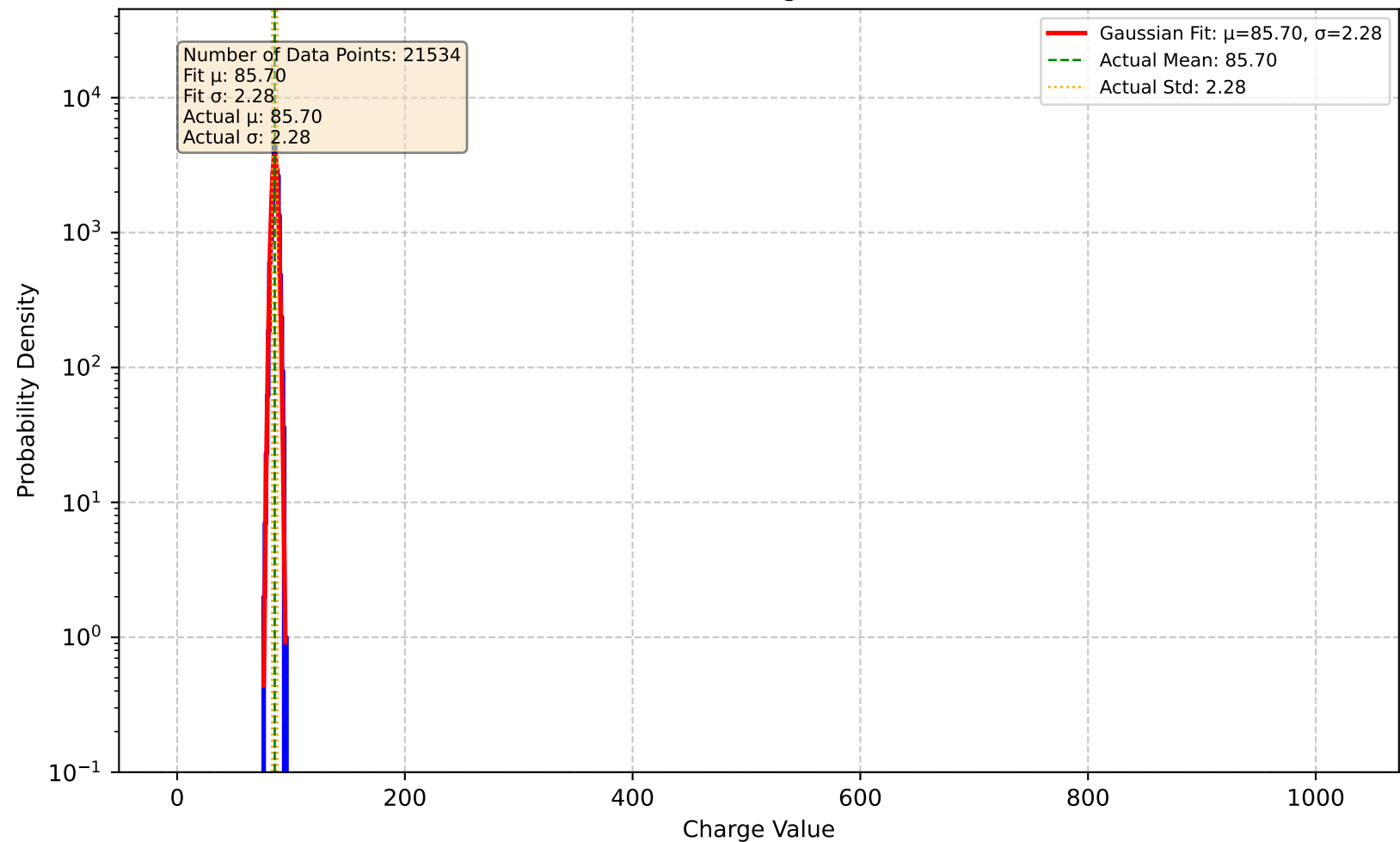
Channel 86 - Charge Distribution
