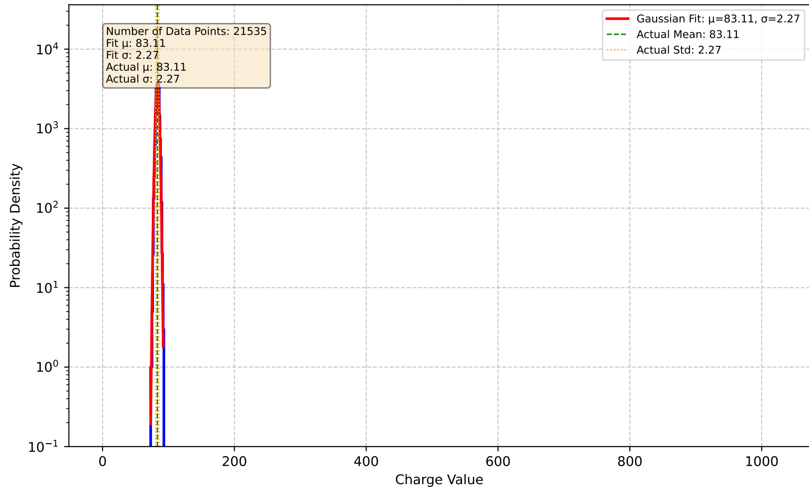
Channel 87 - Charge Distribution
