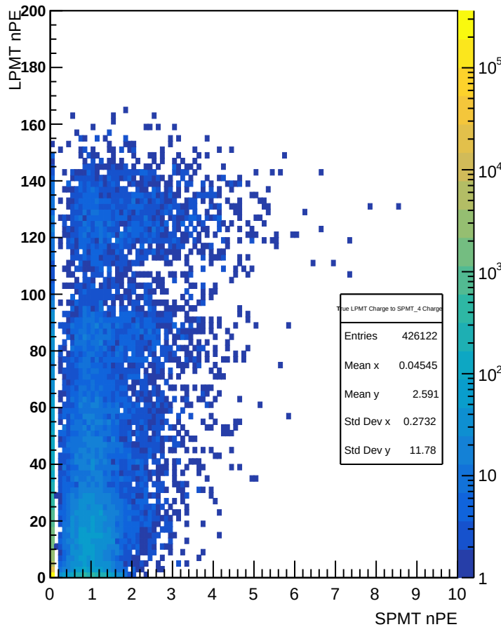
True LPMT Charge to SPMT_4 Charge
