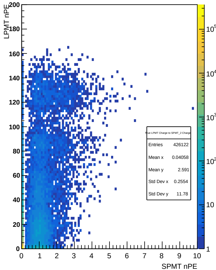
True LPMT Charge to SPMT_2 Charge
