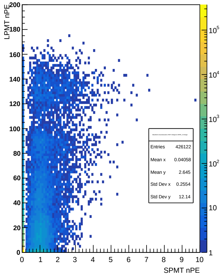
Waveform reconstruction LPMT Charge to SPMT_2 Charge
