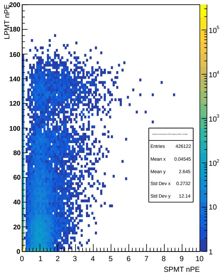
Waveform reconstruction LPMT Charge to SPMT_4 Charge
