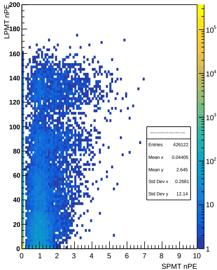
Waveform reconstruction LPMT Charge to SPMT_5 Charge
