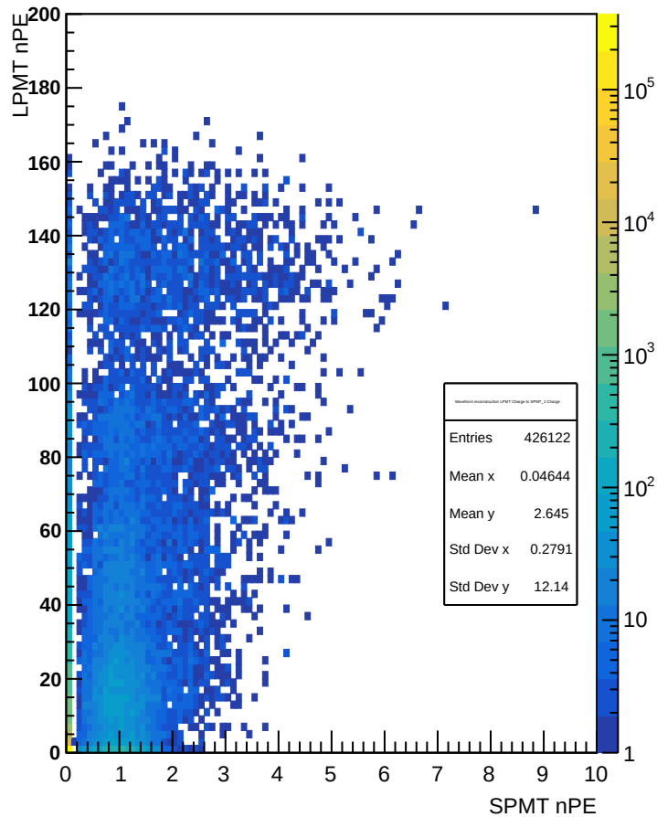
Waveform reconstruction LPMT Charge to SPMT_1 Charge
