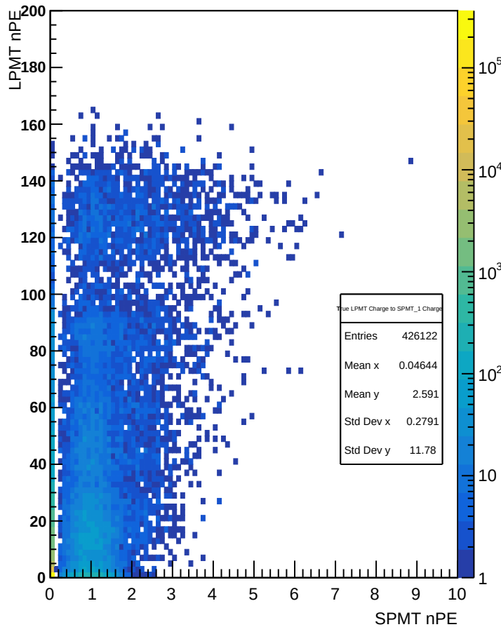
True LPMT Charge to SPMT_1 Charge
