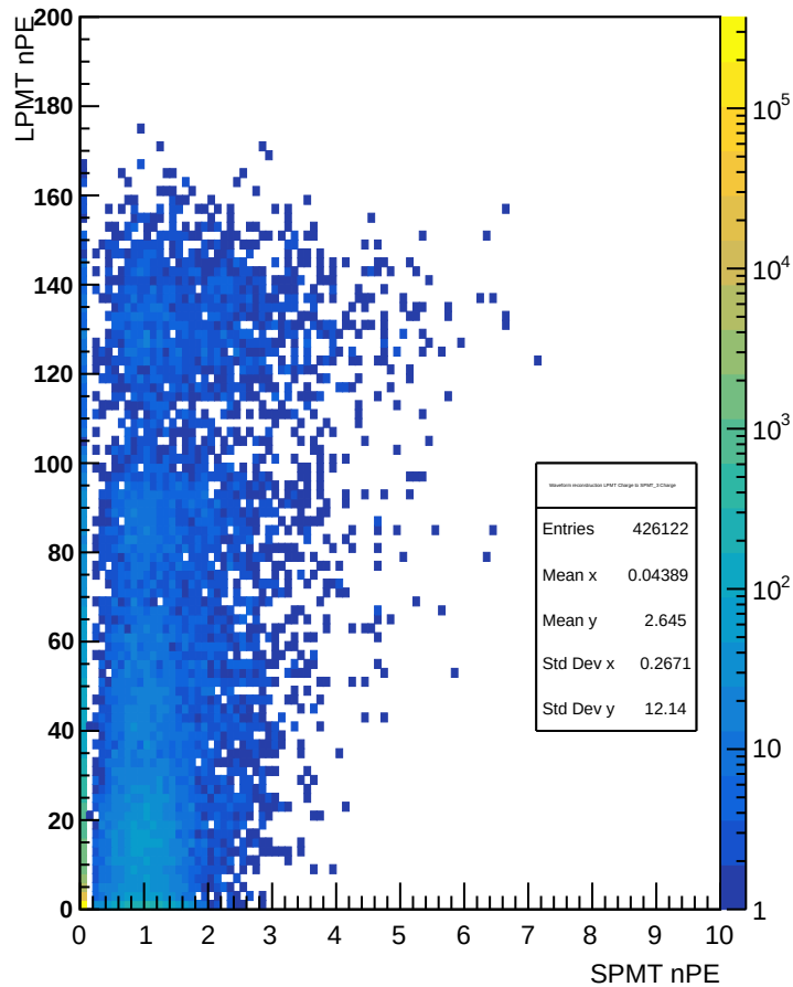
Waveform reconstruction LPMT Charge to SPMT_3 Charge
