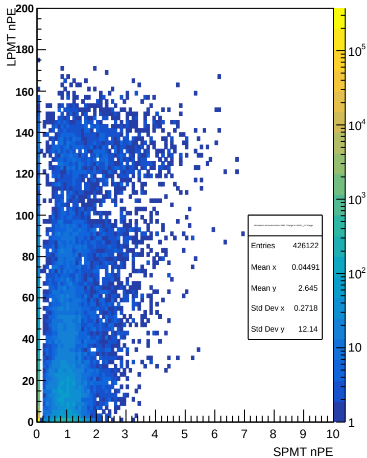
Waveform reconstruction LPMT Charge to SPMT_0 Charge
