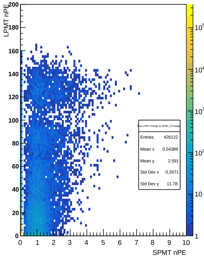
True LPMT Charge to SPMT_3 Charge
