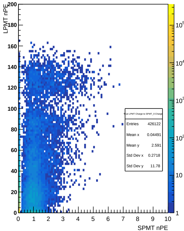
True LPMT Charge to SPMT_0 Charge
