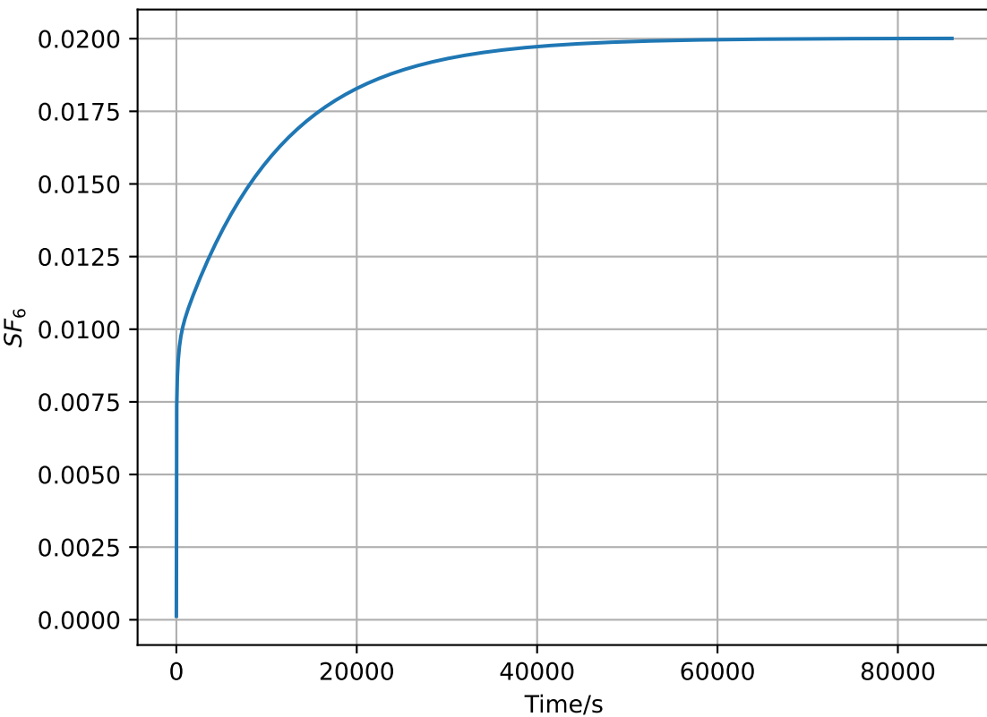
SF_6 concentration at center/ppm
