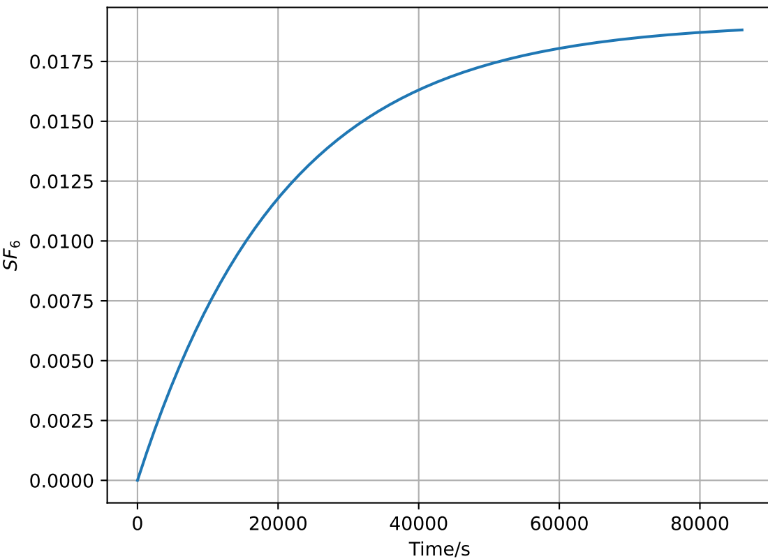
Average SF_6 concentration/ppm
