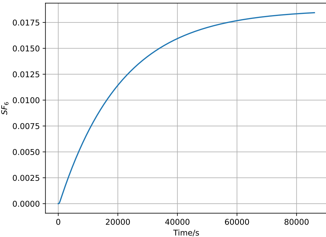
SF_6 concentration at corner/ppm
