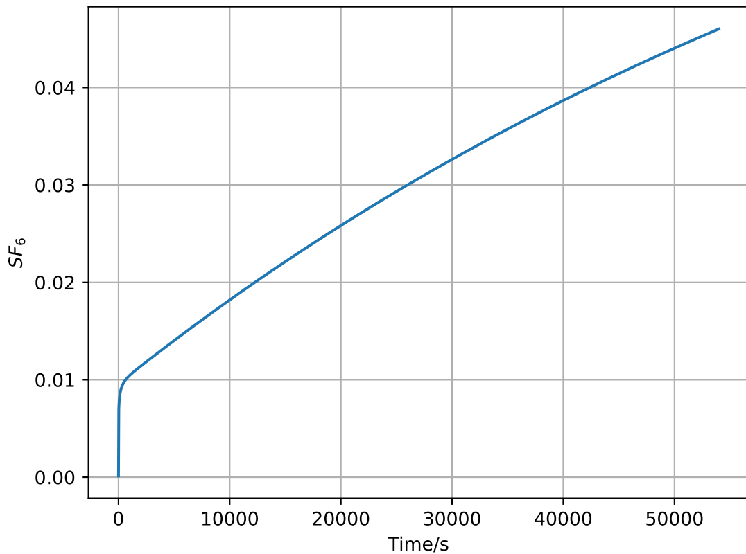
SF_6 concentration at center/ppm
