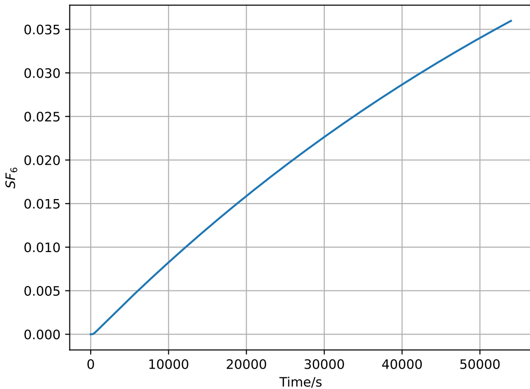
SF_6 concentration at corner/ppm
