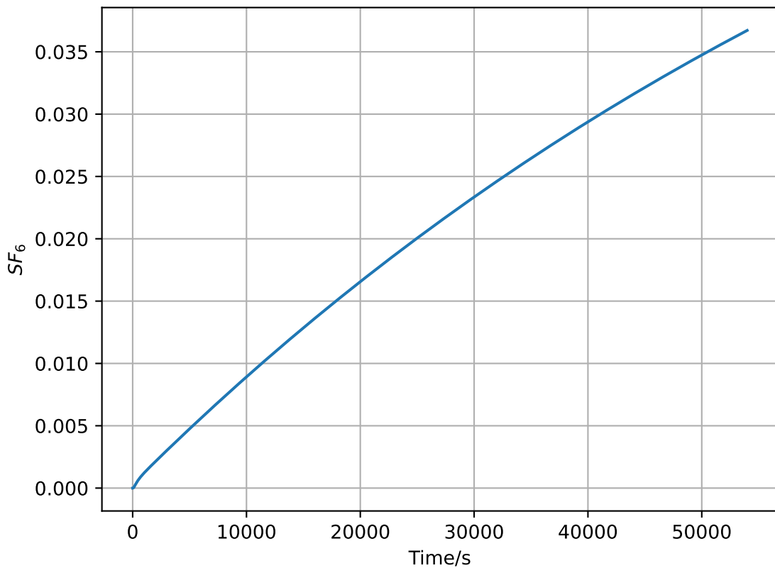
SF_6 concentration at quarter/ppm
