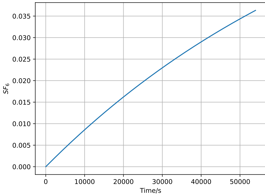
Average SF_6 concentration/ppm
