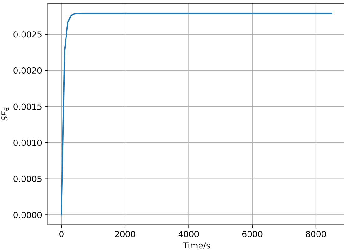
SF_6 concentration at 2cm/ppm
