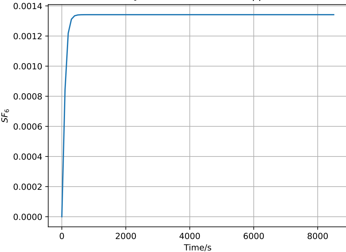
SF_6 concentration at 5cm/ppm
