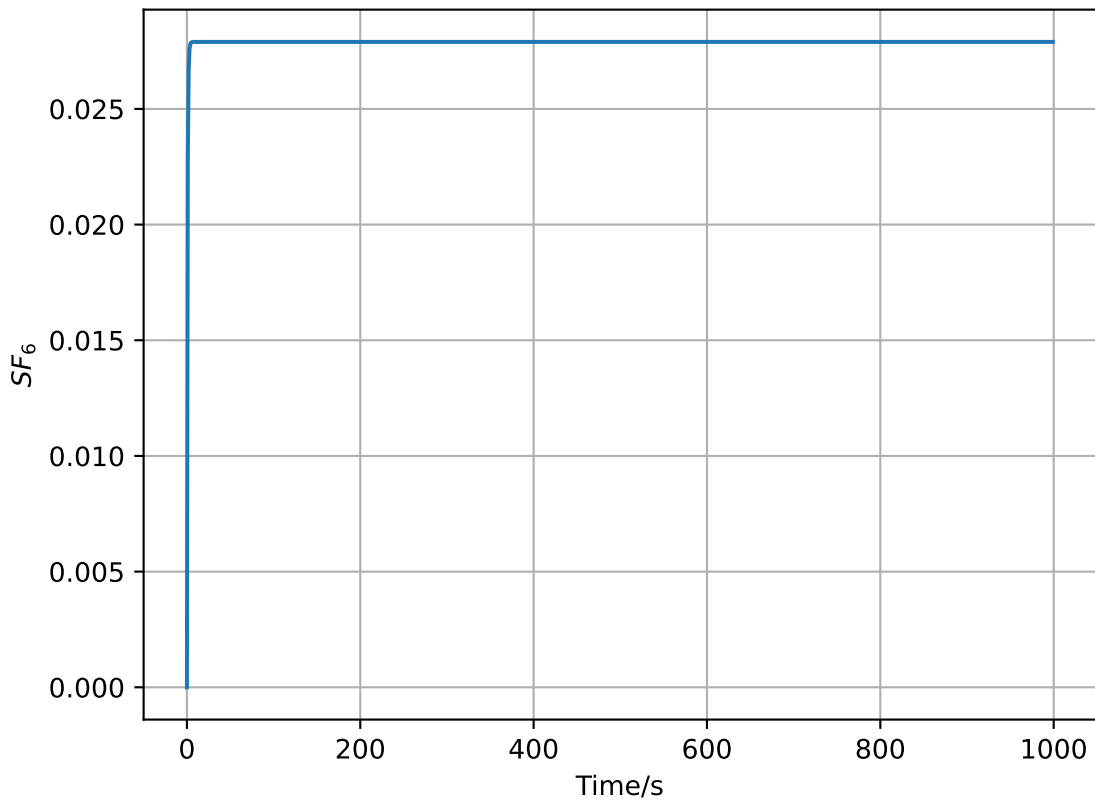
SF_6 concentration at 2mm/ppm
