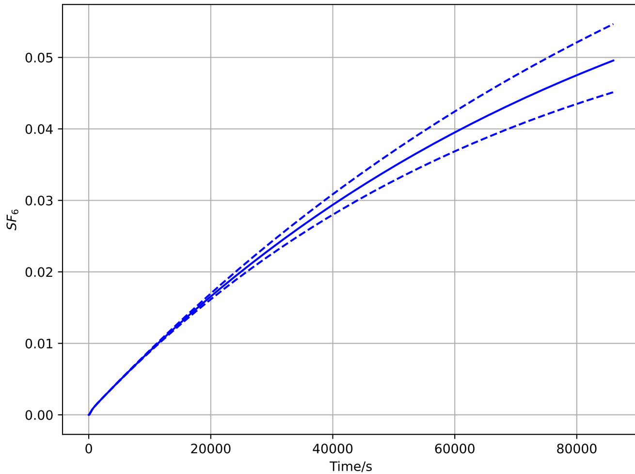
SF_6 concentration at quarter/ppm
