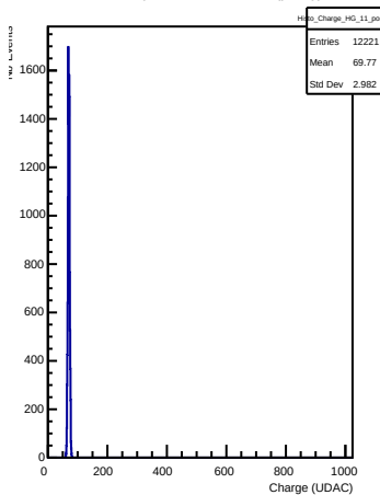
HG Charges in channel 11 (pong)
