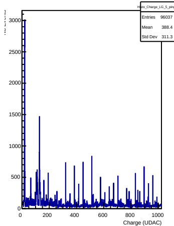
LG Charges in channel 5 (ping)
