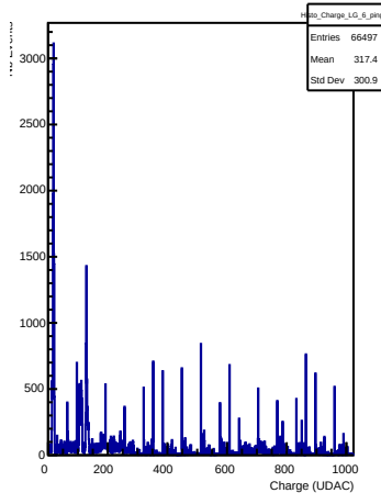
LG Charges in channel 6 (ping)
