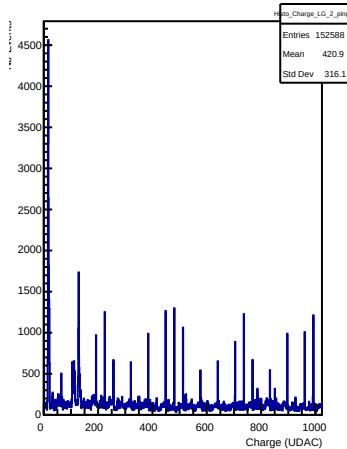
LG Charges in channel 2 (ping)
