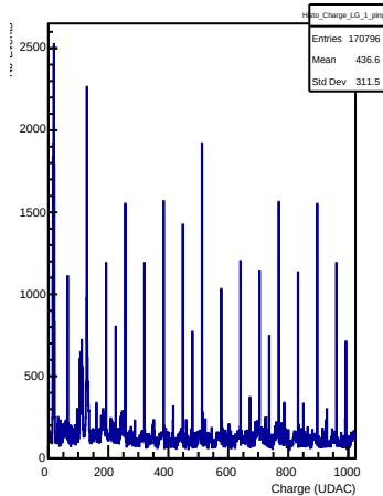
LG Charges in channel 1 (ping)
