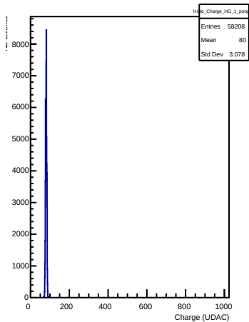
HG Charges in channel 1 (pong)
