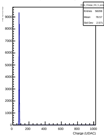
HG Charges in channel 5 (pong)
