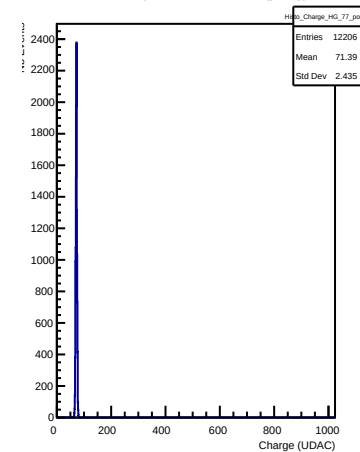
HG Charges in channel 77 (pong)
