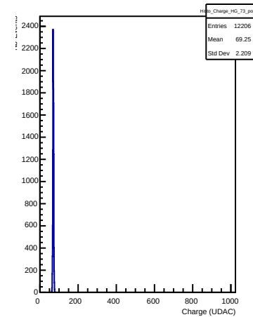
HG Charges in channel 73 (pong)
