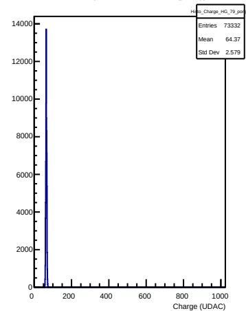
HG Charges in channel 79 (pong)
