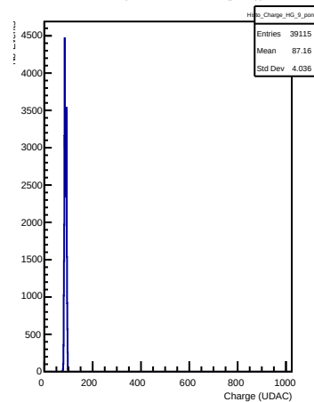
HG Charges in channel 9 (pong)
