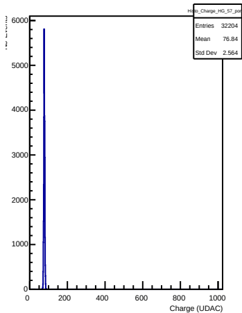
HG Charges in channel 57 (pong)
