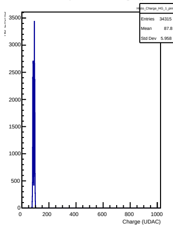
HG Charges in channel 1 (ping)
