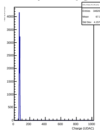
HG Charges in channel 108 (pong)
