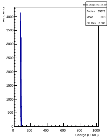
HG Charges in channel 19 (pong)
