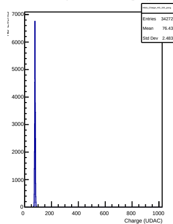
HG Charges in channel 104 (pong)
