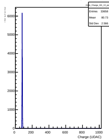
HG Charges in channel 13 (pong)
