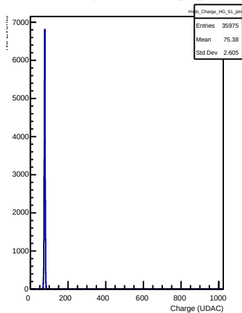
HG Charges in channel 61 (ping)
