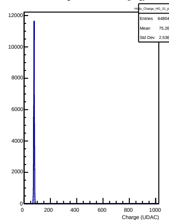
HG Charges in channel 31 (ping)
