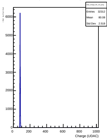
HG Charges in channel 113 (pong)
