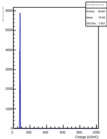
HG Charges in channel 117 (pong)
