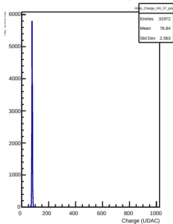
HG Charges in channel 57 (ping)
