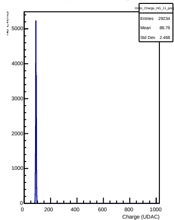
HG Charges in channel 11 (pong)
