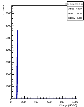
HG Charges in channel 15 (pong)
