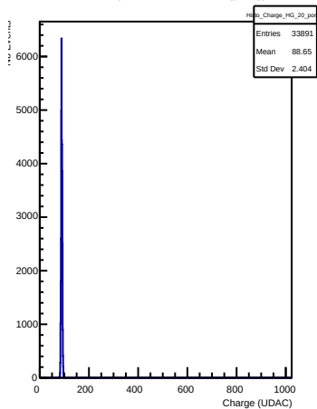
HG Charges in channel 20 (pong)
