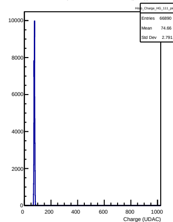
HG Charges in channel 111 (ping)
