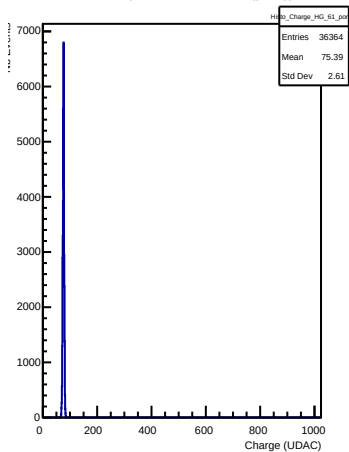
HG Charges in channel 61 (pong)
