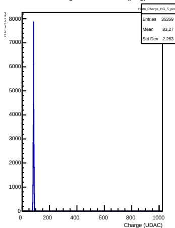
HG Charges in channel 5 (ping)
