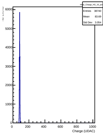
HG Charges in channel 16 (pong)
