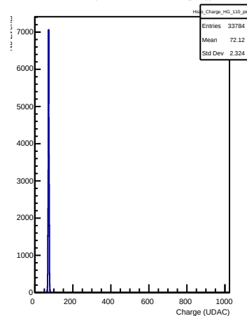
HG Charges in channel 110 (ping)
