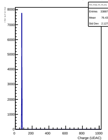
HG Charges in channel 118 (pong)
