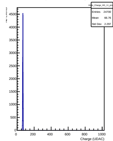
HG Charges in channel 11 (ping)
