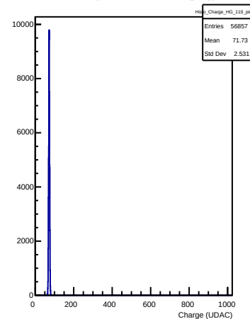
HG Charges in channel 119 (ping)
