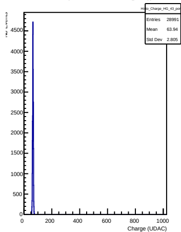
HG Charges in channel 43 (pong)
