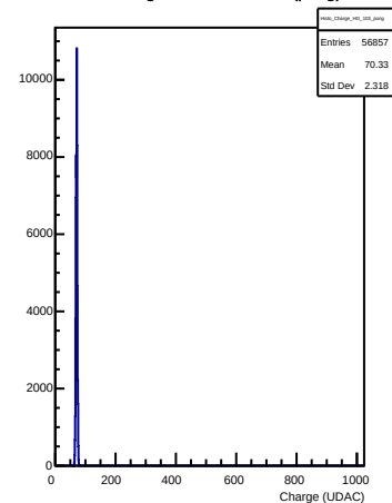
HG Charges in channel 103 (pong)
