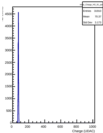
HG Charges in channel 81 (pong)
