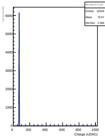
HG Charges in channel 117 (pong)
