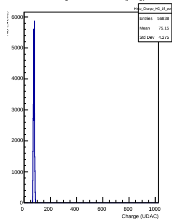
HG Charges in channel 15 (pong)
