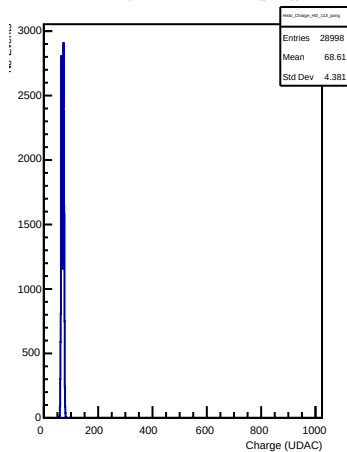
HG Charges in channel 113 (pong)
