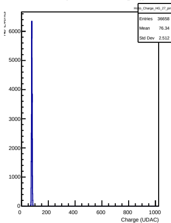
HG Charges in channel 27 (ping)
