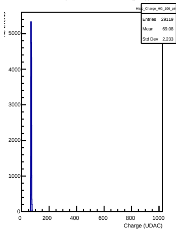
HG Charges in channel 106 (ping)
