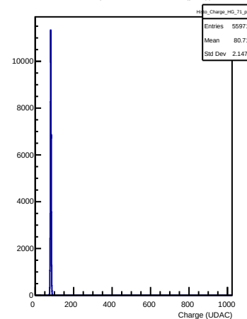
HG Charges in channel 71 (ping)
