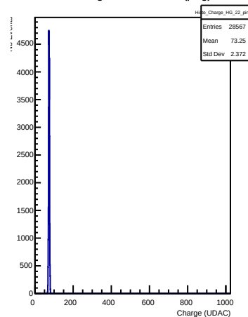
HG Charges in channel 22 (ping)
