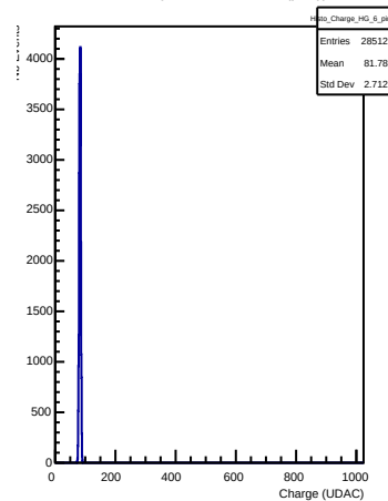
HG Charges in channel 6 (ping)
