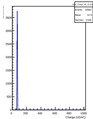
HG Charges in channel 46 (pong)
