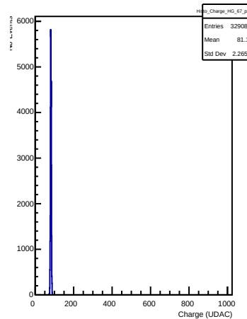
HG Charges in channel 67 (ping)
