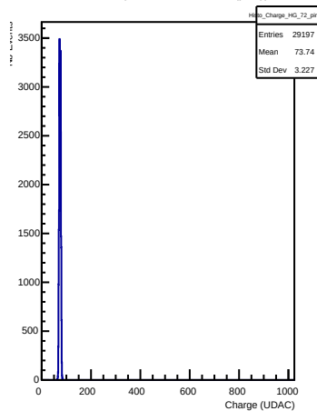
HG Charges in channel 72 (ping)
