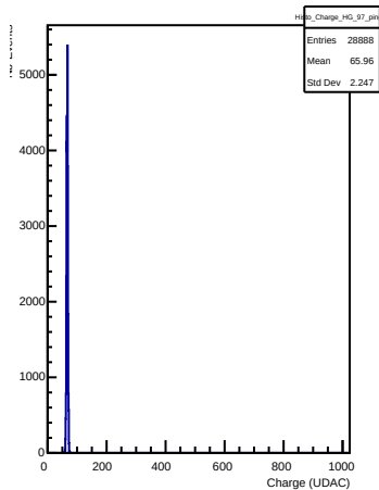
HG Charges in channel 97 (ping)
