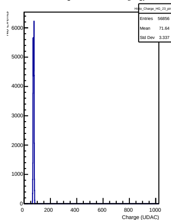
HG Charges in channel 23 (ping)
