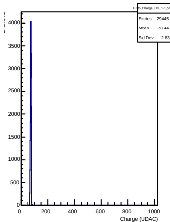
HG Charges in channel 17 (pong)
