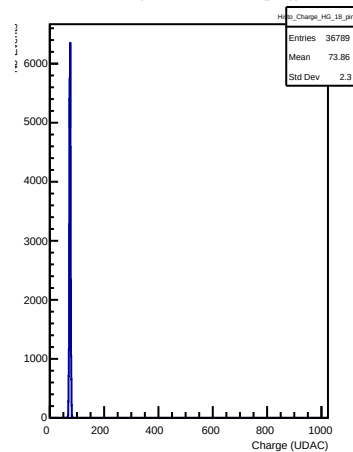
HG Charges in channel 18 (ping)
