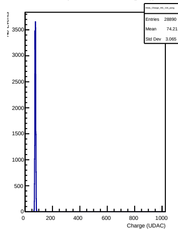
HG Charges in channel 115 (pong)
