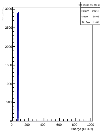
HG Charges in channel 113 (ping)
