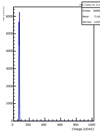
HG Charges in channel 23 (pong)
