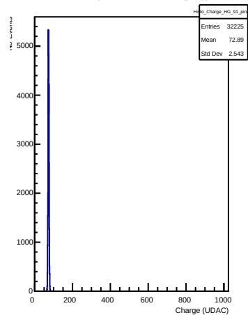
HG Charges in channel 91 (ping)
