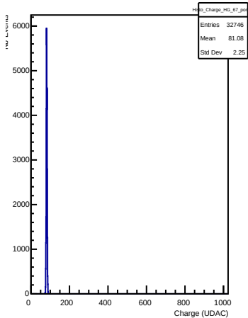
HG Charges in channel 67 (pong)
