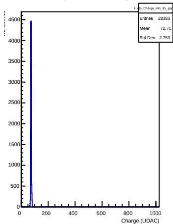
HG Charges in channel 85 (pong)
