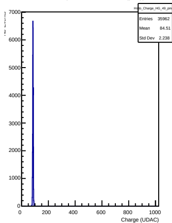
HG Charges in channel 49 (ping)
