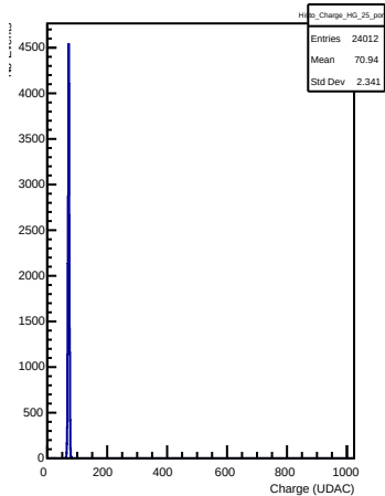
HG Charges in channel 25 (pong)
