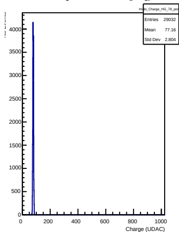
HG Charges in channel 78 (pong)
