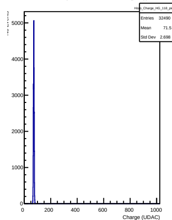
HG Charges in channel 118 (ping)
