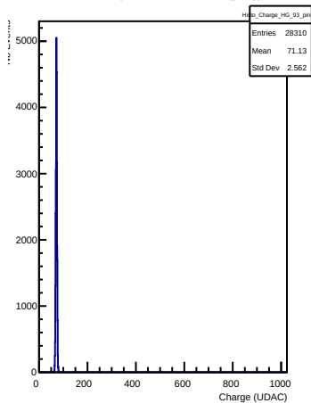
HG Charges in channel 93 (ping)
