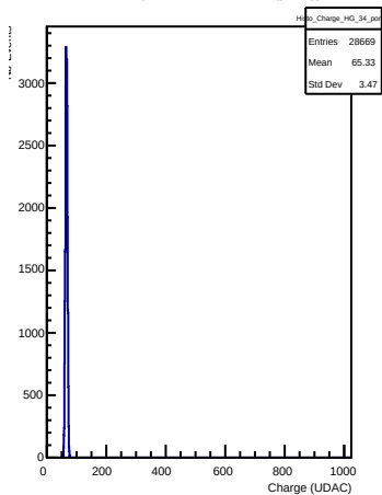
HG Charges in channel 34 (pong)
