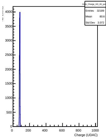
HG Charges in channel 65 (pong)
