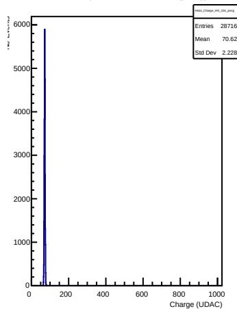
HG Charges in channel 104 (pong)
