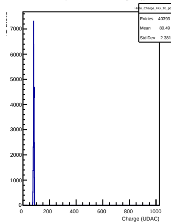
HG Charges in channel 10 (pong)
