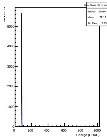
HG Charges in channel 3 (pong)
