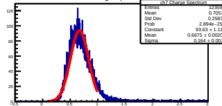
ch7 Charge Spectrum
