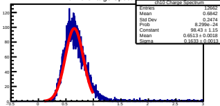
ch10 Charge Spectrum
