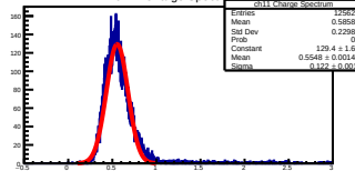
ch11 Charge Spectrum
