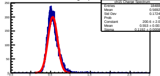
ch15 Charge Spectrum
