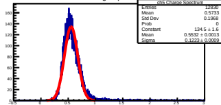
ch5 Charge Spectrum
