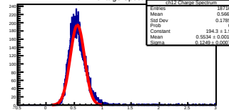
ch12 Charge Spectrum
