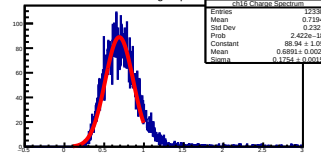
ch16 Charge Spectrum
