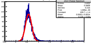
ch14 Charge Spectrum
