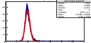
ch13 Charge Spectrum
