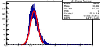
ch1 Charge Spectrum
