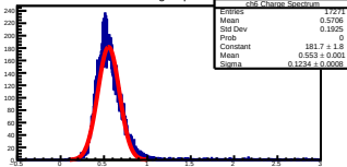
ch6 Charge Spectrum
