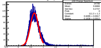
ch9 Charge Spectrum
