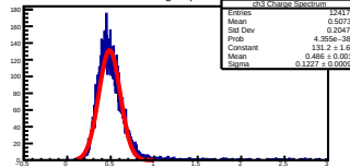
ch3 Charge Spectrum
