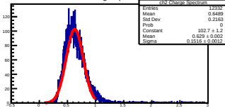
ch2 Charge Spectrum
