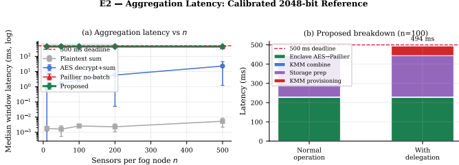
Fig. 4. E2: Aggregation latency vs sensor count n with calibrated 2048-bit host-reference Paillier timings. The dashed line marks the 500 ms window. The right panel shows the calibrated component breakdown of the proposed method.
