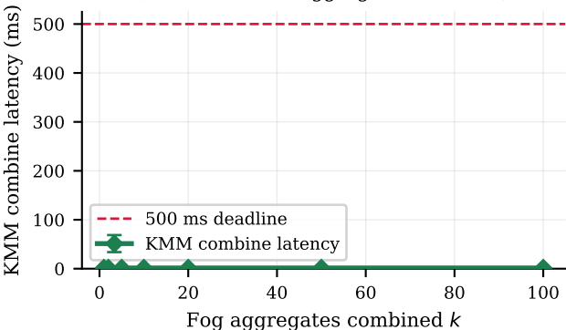
E4 — KMM Window-Combine Overhead (calibrated host aggregate reference)
