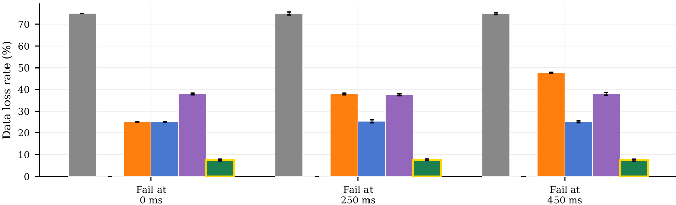
E6 — Data Loss Rate by Method and Failure Time (lower = better; gold border = Proposed; 95% CI bars; analytical model, 30 seeds)
