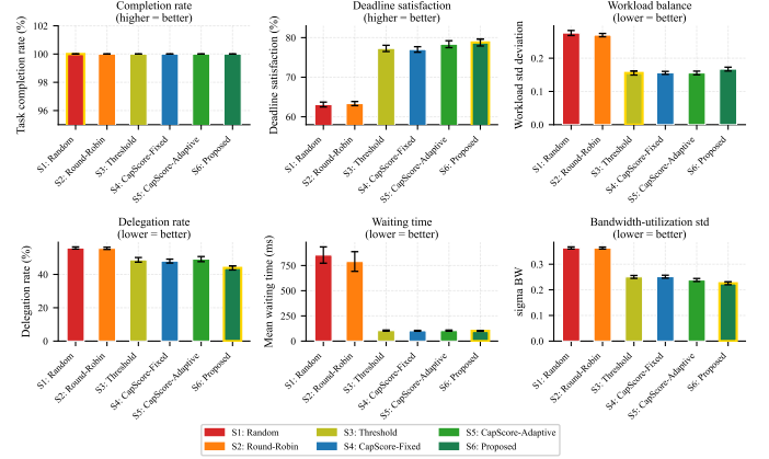
Fig. 6. Six-strategy load-balancing comparison: completion rate, deadline satisfaction, delegation rate, mean waiting time, and bandwidth-utilization standard deviation over 20 seeds with 95% CI.
