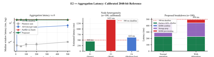
Fig. 4. Aggregation latency vs sensor count n with calibrated 2048-bit host-reference Paillier timings. The dashed line marks 500 ms. The right panel shows the component breakdown.
