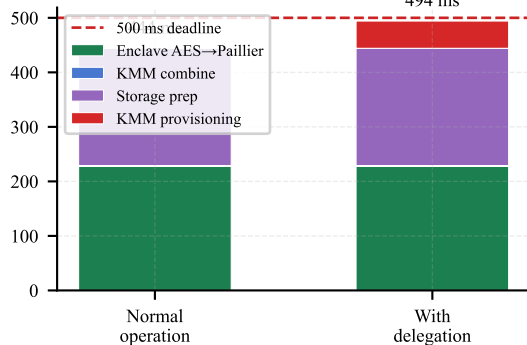
Proposed breakdown ( n=100 )
