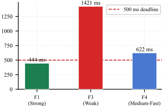
Node heterogeneity ( n=100 , calibrated)
