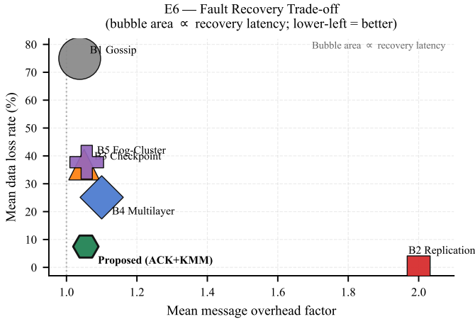
Fig. 9. Data loss vs message overhead tradeoff. The proposed ACK+KMM method (green) is closest to the origin among single-mechanism approaches.
