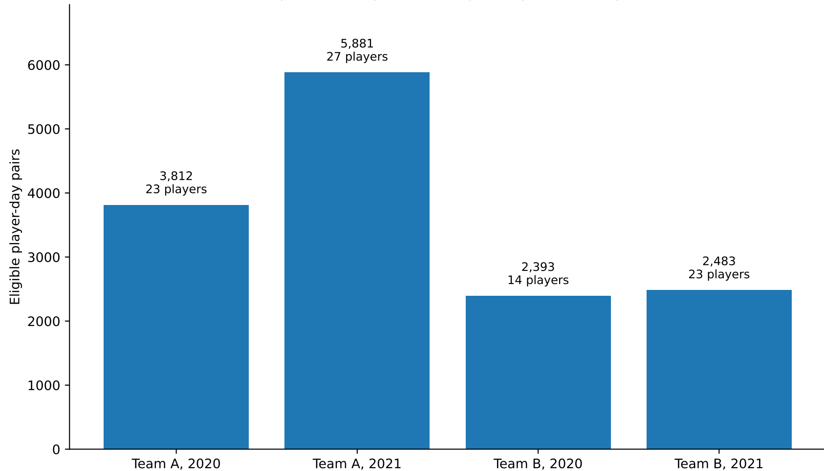
Analytic next-day readiness pairs by team and year
